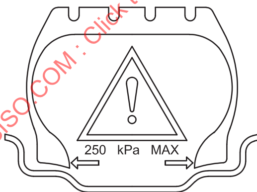
Figure 1 — Example of pictogram of maximum inflation pressure for bead seating
