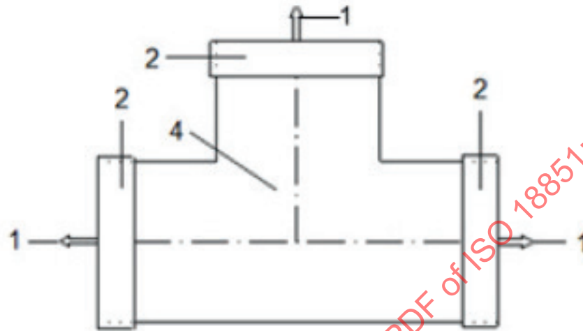
a) Arrangement with end loads
