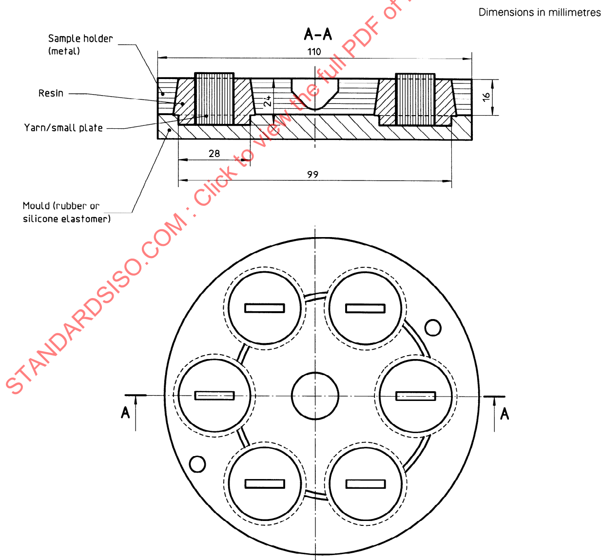
Figure 1 — Example of assembly for moulding specimens
