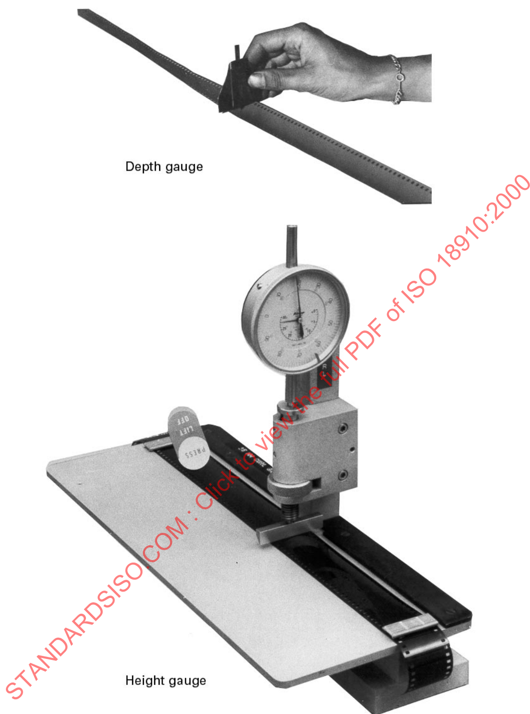
Figure 3 — Devices for reading edge curl of film strips for test method B
