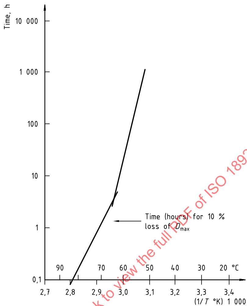
Figure C.1 — Arrhenius plot of D_{\max} loss of a vesicular film [20]
