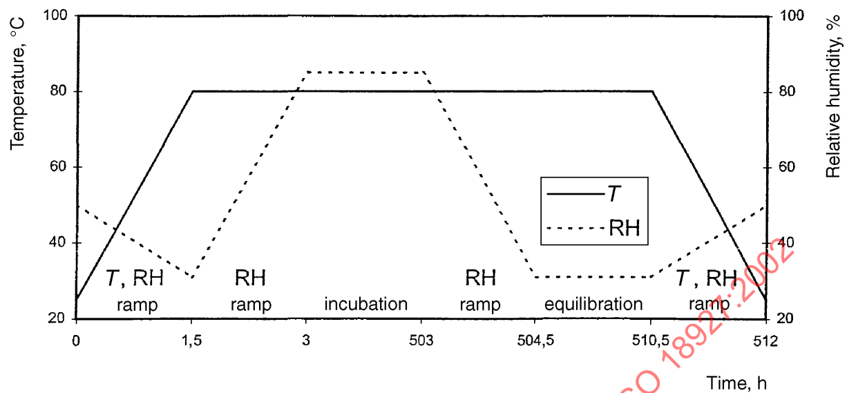
Figure 1 — Graph of nominal 80 °C/85 % RH transition (ramp) profile (as per Tables 1 and 2)
