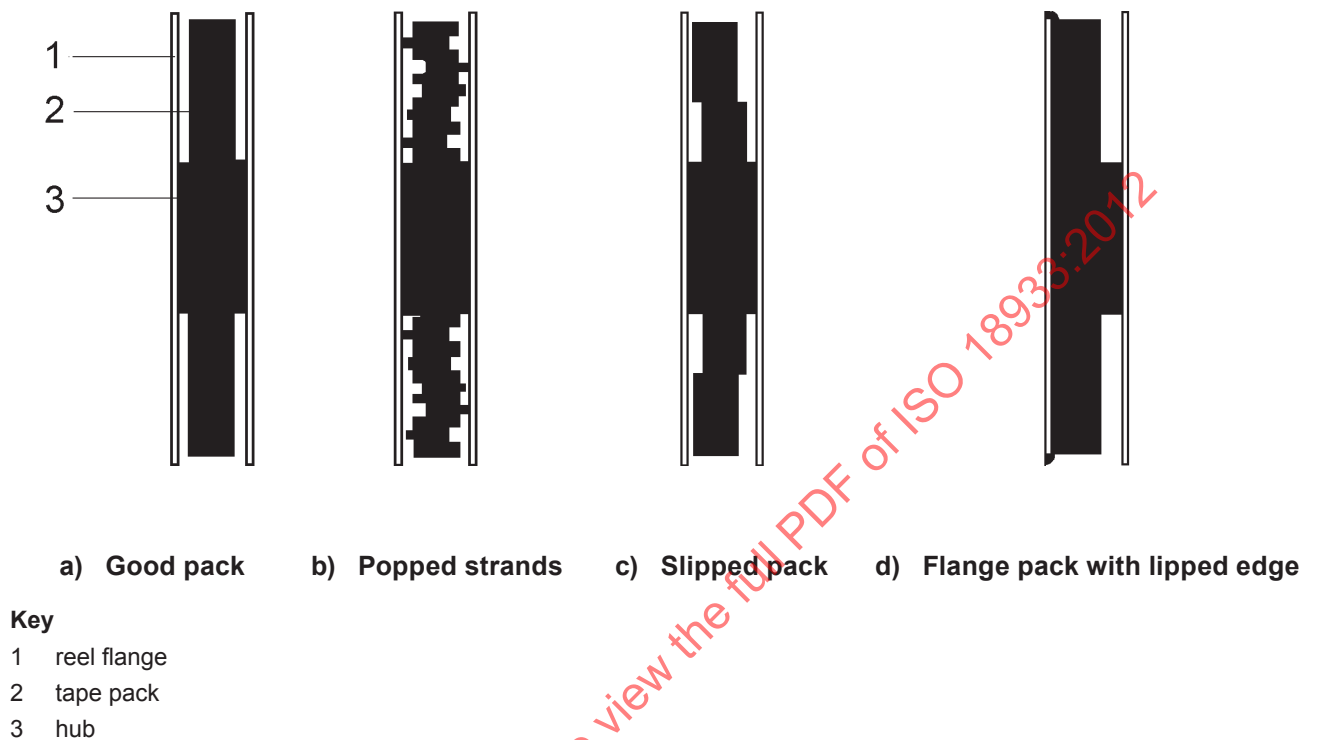
Figure 1 — Examples of tape packs
