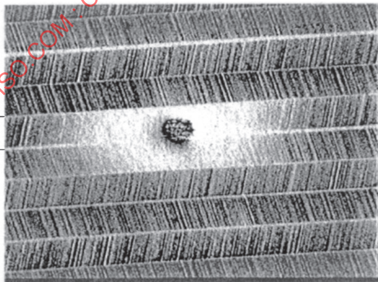
Figure 3 — Loss of data due to a clump of debris on the surface of the tape
