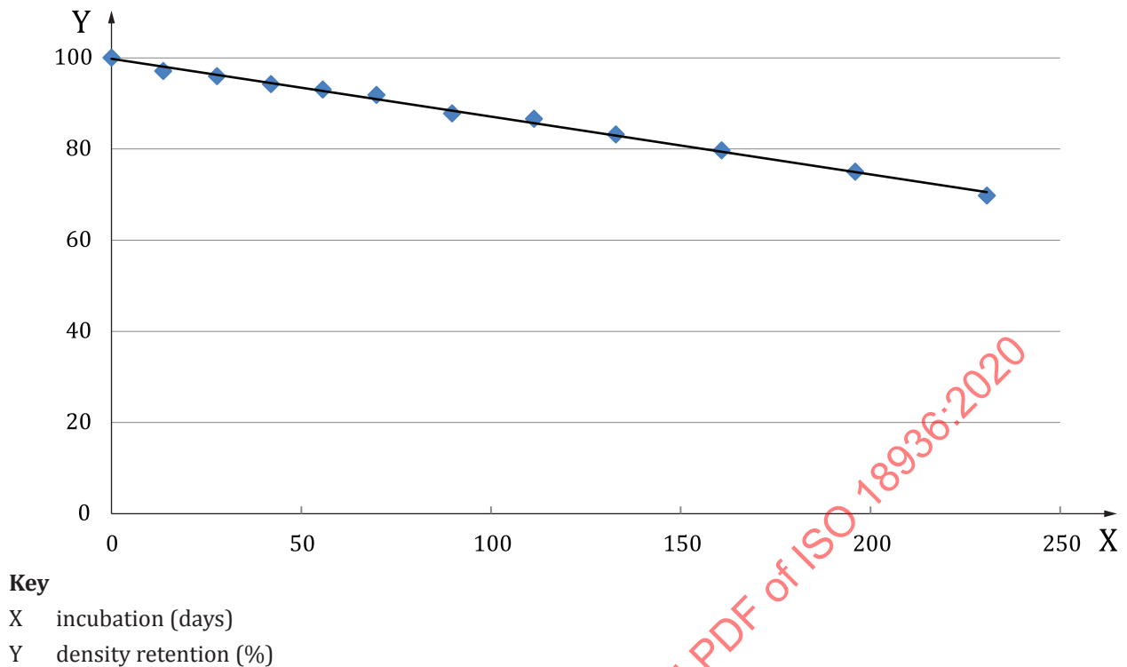
Figure A.1 — Density versus time of incubation (at 60 °C)
