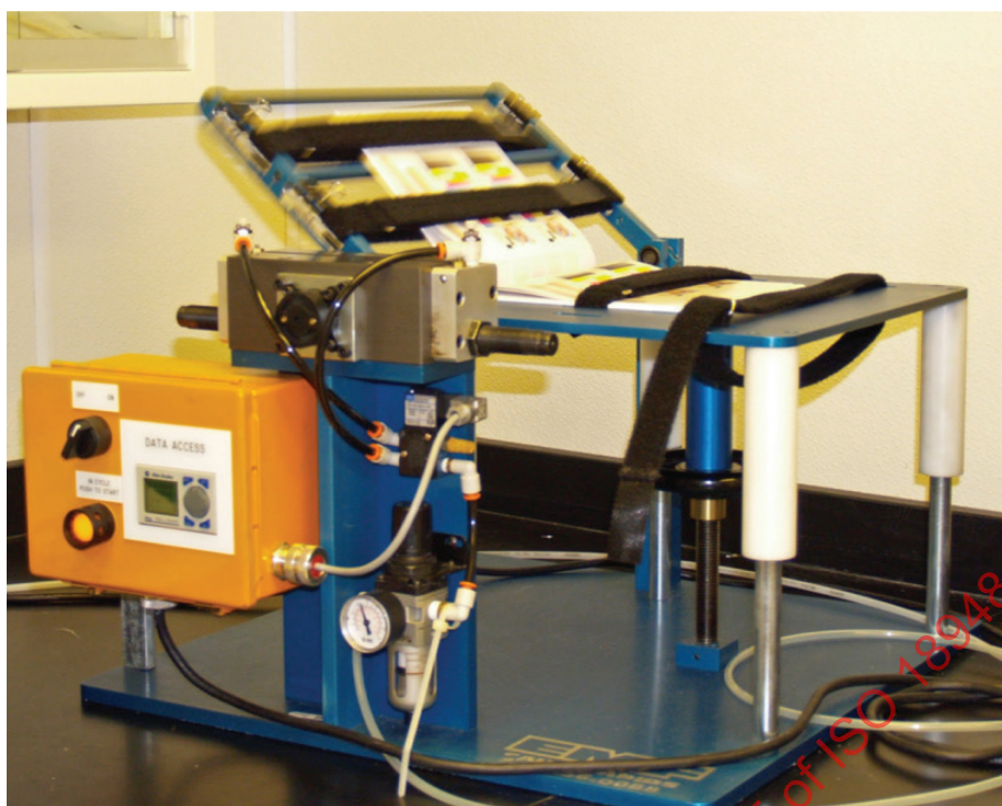
Figure 1 — Example of a page turner device for use in the open-close test
