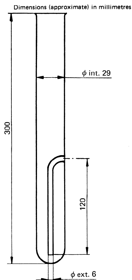
FIGURE 3 — Bubbler tube (C)
