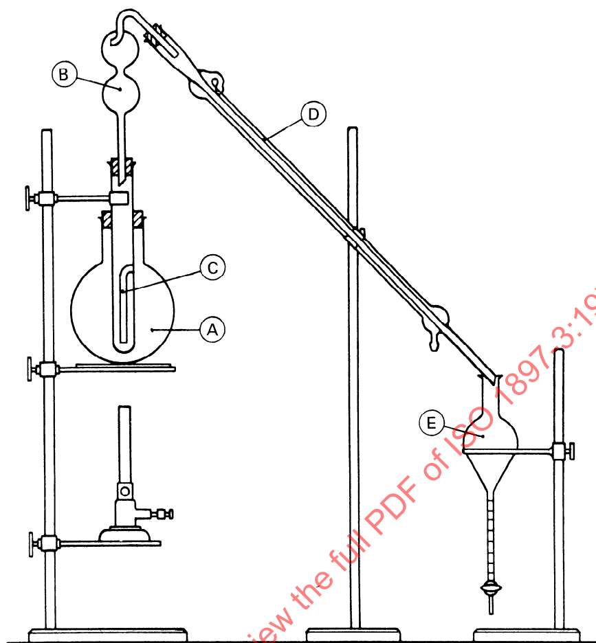
FIGURE 1 — Assembled distillation apparatus
