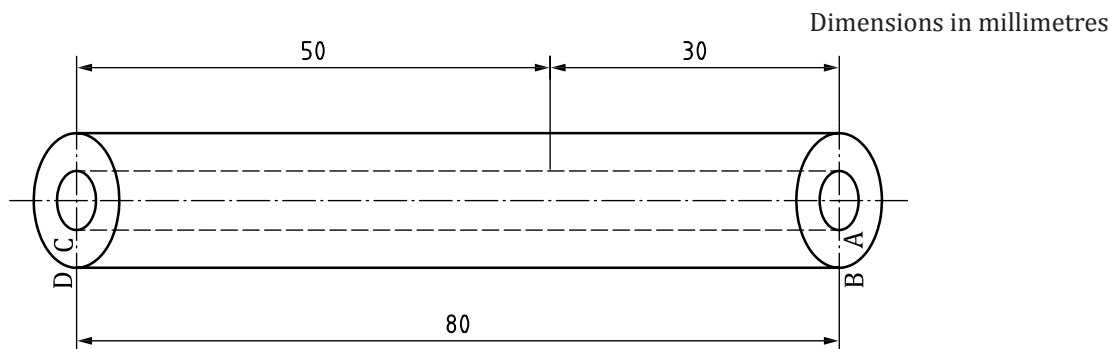
Figure B.1 — Shape and dimensions of the test piece
