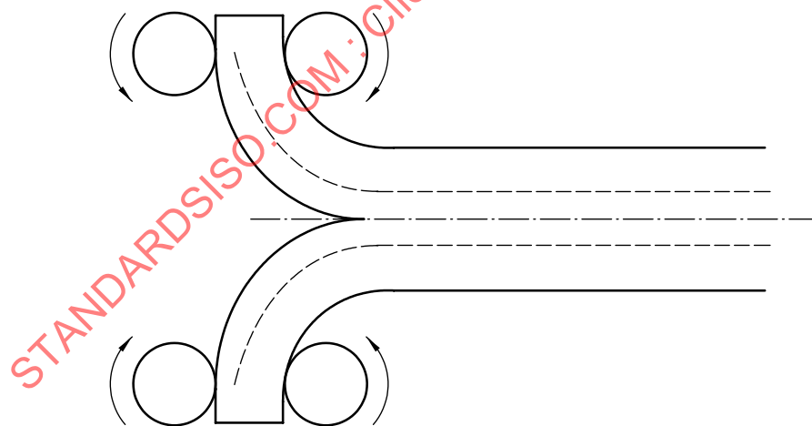
Figure B.2 — Position of the test piece in the grips
