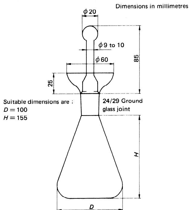
FIGURE — 500 ml iodine flask (5.1)
