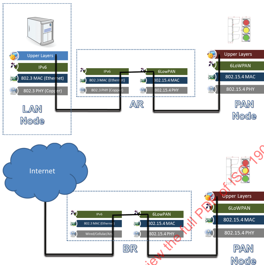
Figure 2 — 6LoWPAN subsystem
