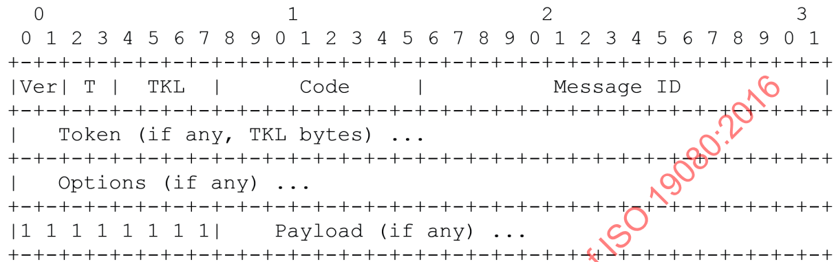
Figure 7 — Message format
