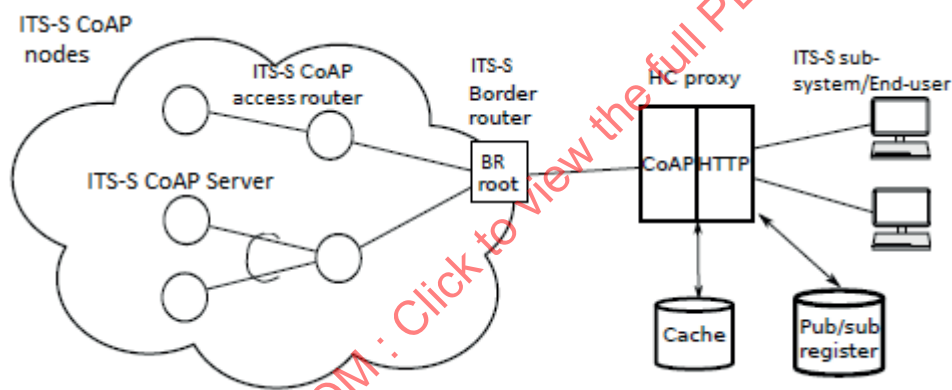
Figure 12 — Example caching architecture in ITS-S
