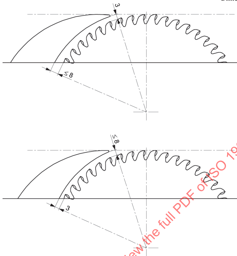
Figure 10 — Positioning limits for riving knife design
