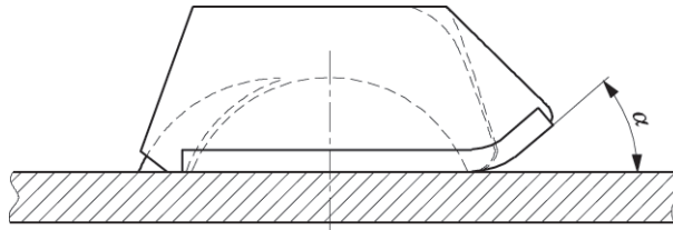
Figure 5 — Design of the “lead-in”
