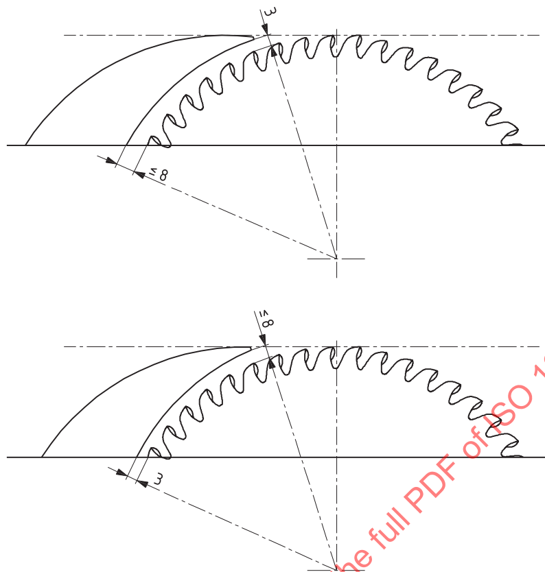
Figure 22 — Riving knife positioning limits
