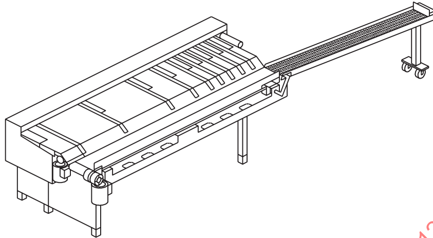
Figure 10 — Example of automatic work-piece returner for a single end machine
