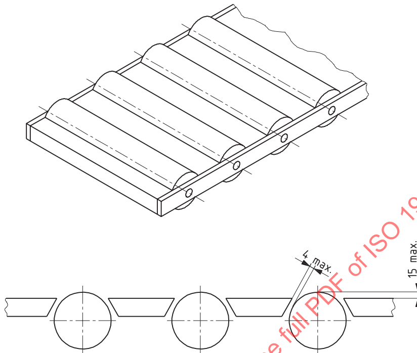
Figure 24 — Safeguarding of gaps between the rollers
