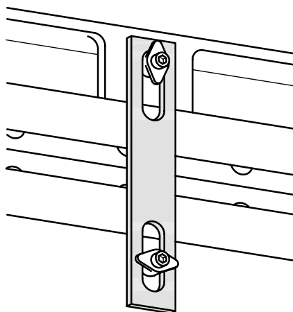
Figure 15 — Example of mechanical platen lock
