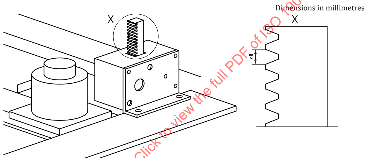
Figure 17 — Example of guarding of the rack
