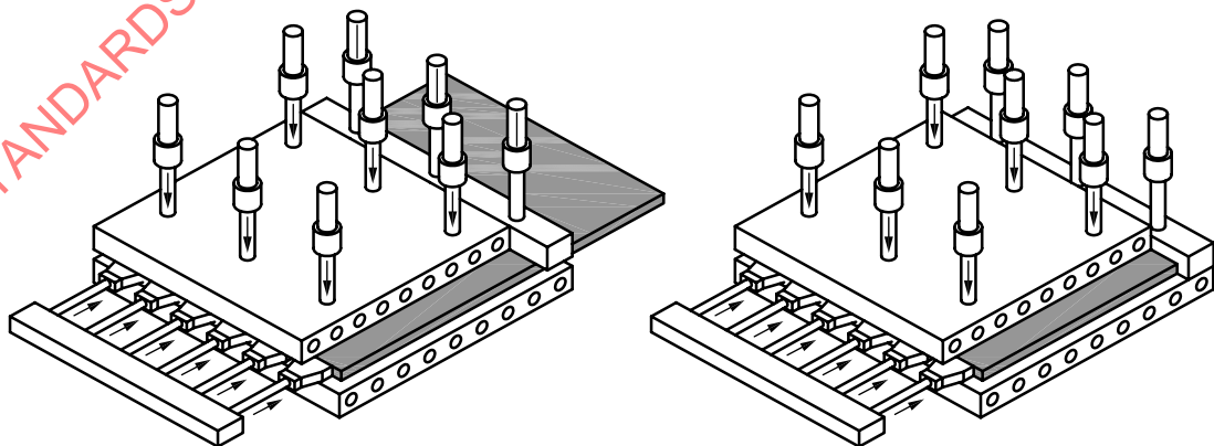
Figure 13 — Examples of automatic work-piece clamping pressure beam
