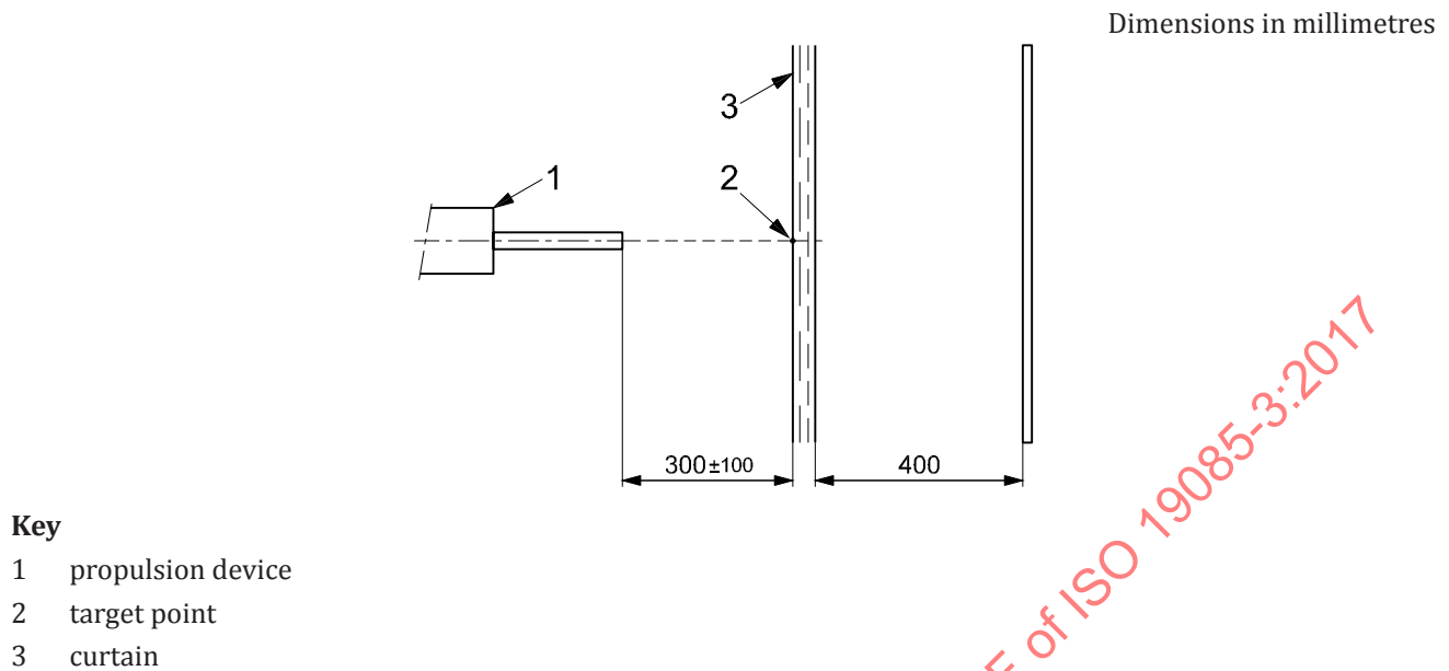
Figure F.1 — Top view of the test arrangement for straight curtains
