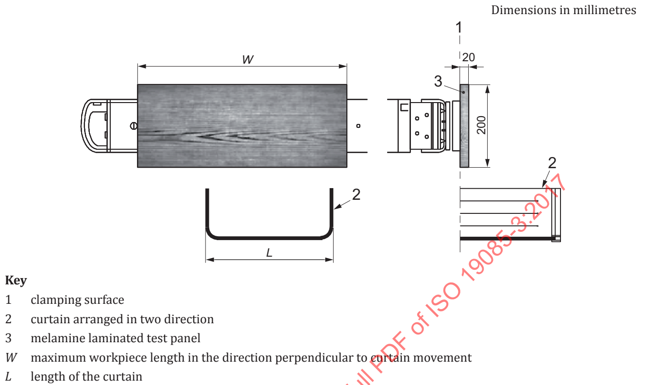
Figure G.2 — Melamine laminated test panels and curtain arranged in two directions
