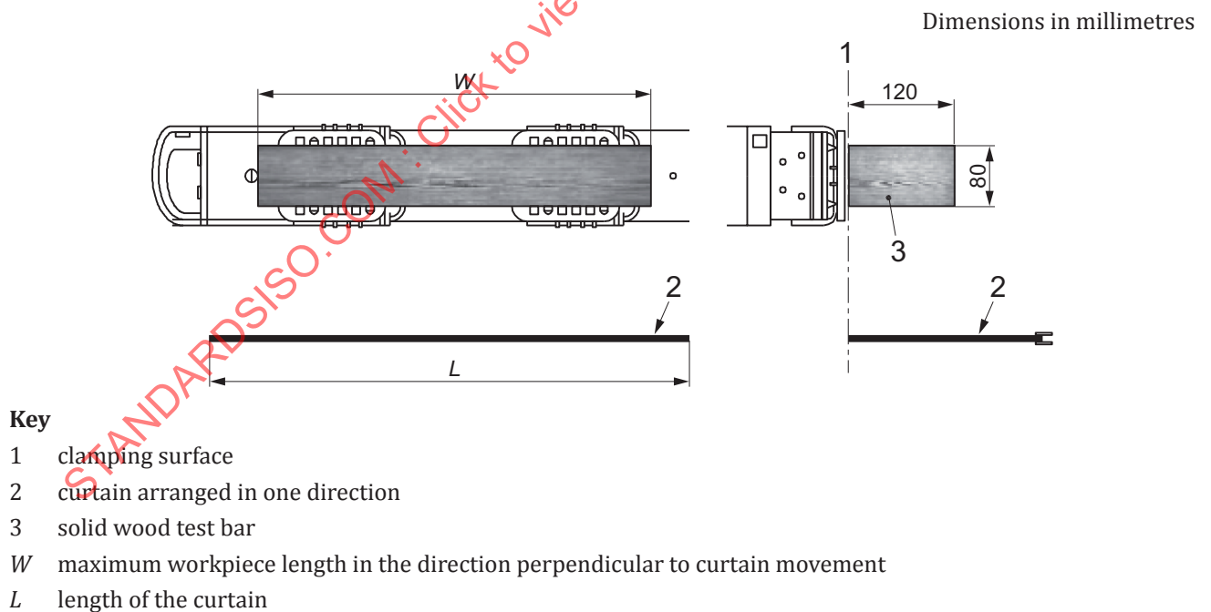
Figure G.3 — Solid wood test bars and curtain arranged in one direction
