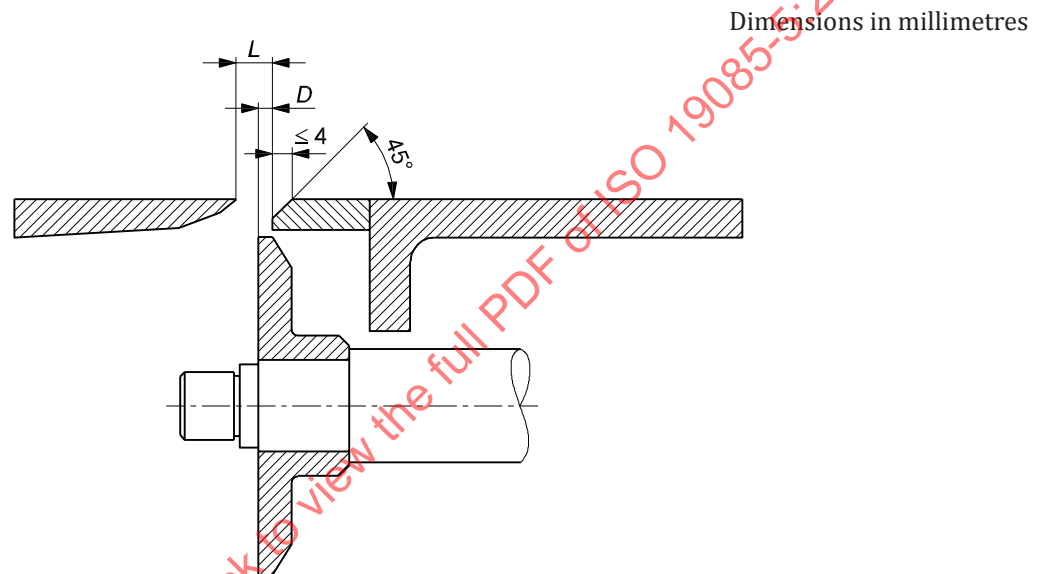
Figure 12 — Width of table slot and distance of fixed saw flange from edge of table slot
