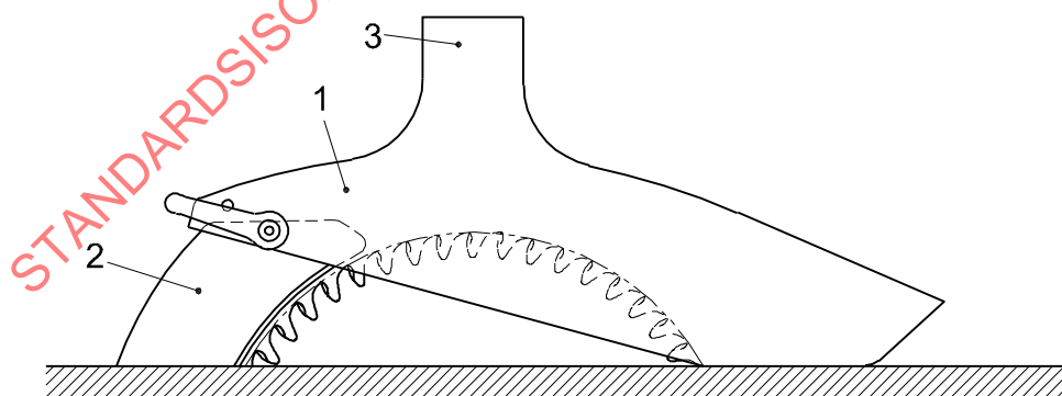
Figure 5 — Example of replaceable ribs at the underside of saw blade guard side walls
