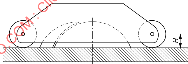
Figure 9 — Dimensions of “lead-in” at front edge of saw blade guards mounted on table separately from riving knife
