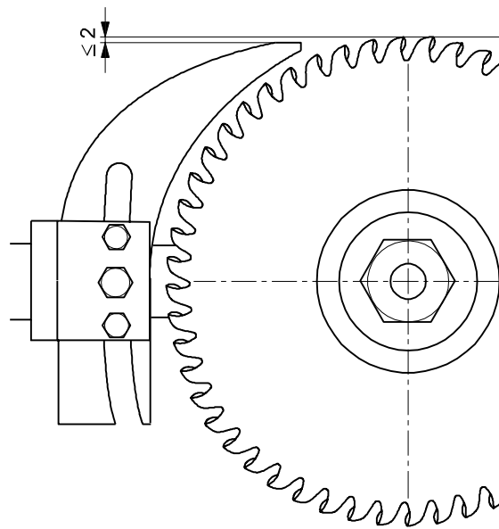
Figure 14 — Riving knife height adjustment
