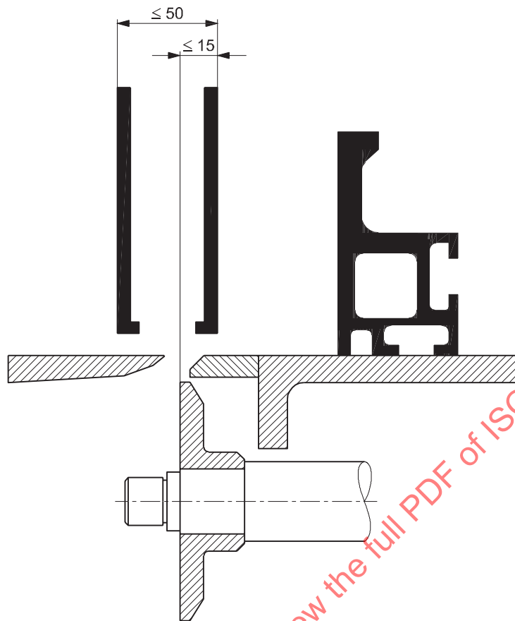
Figure 11 — Maximum width of saw blade guard on machines with saw blade guard mounted separately from riving knife and with non-tilting saw blade
