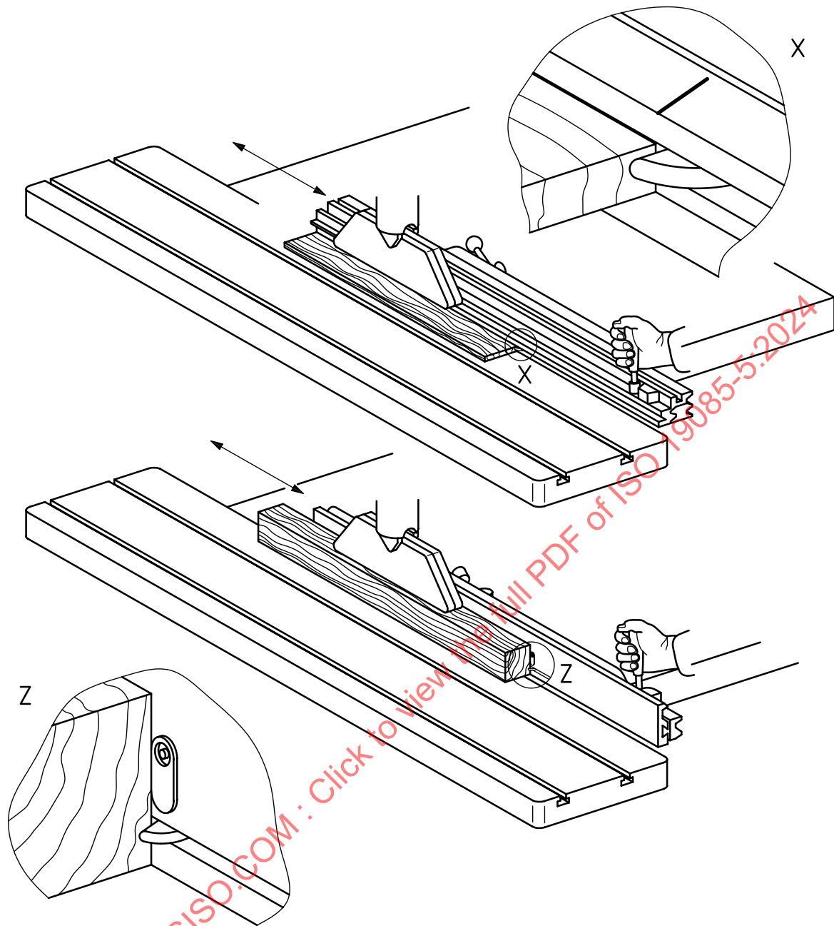
Figure 22 — Example 1 of a safety device for cutting
