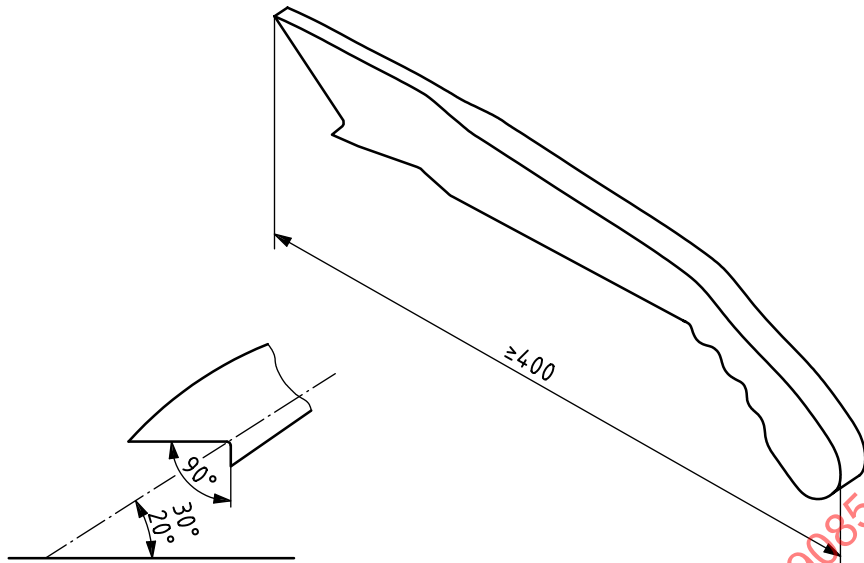
Figure 20 — Example of a push stick
