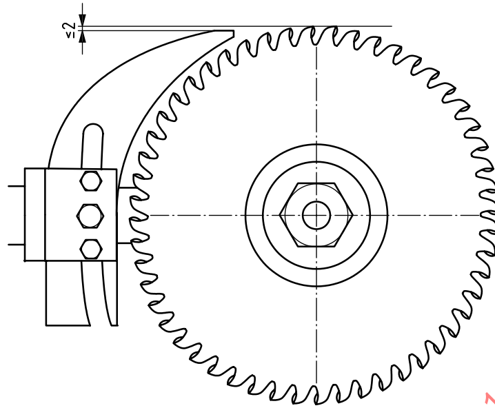
Figure 12 — Riving knife height adjustment
