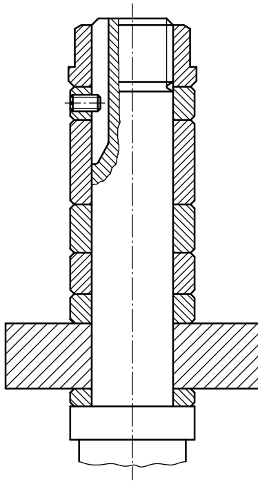
a) Example of an arbor nut
