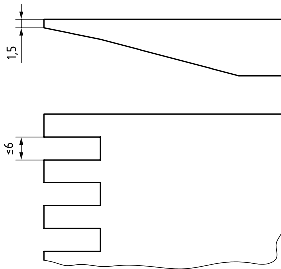
Figure 15 — Example of slots in table lips
