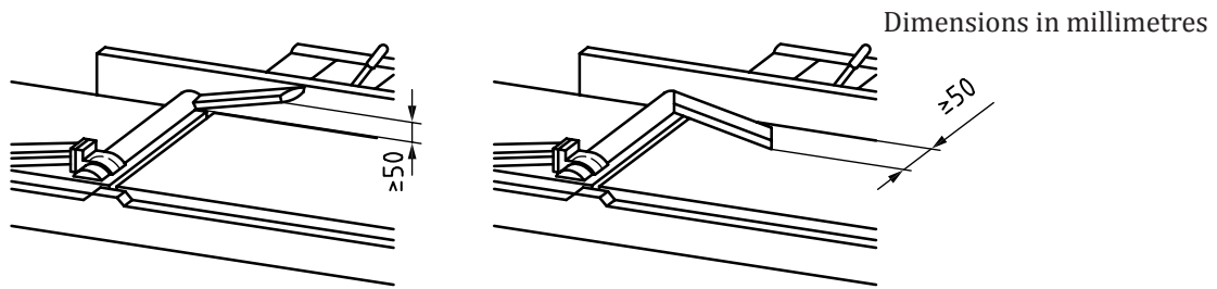
Figure 12 — Examples of leading in devices
