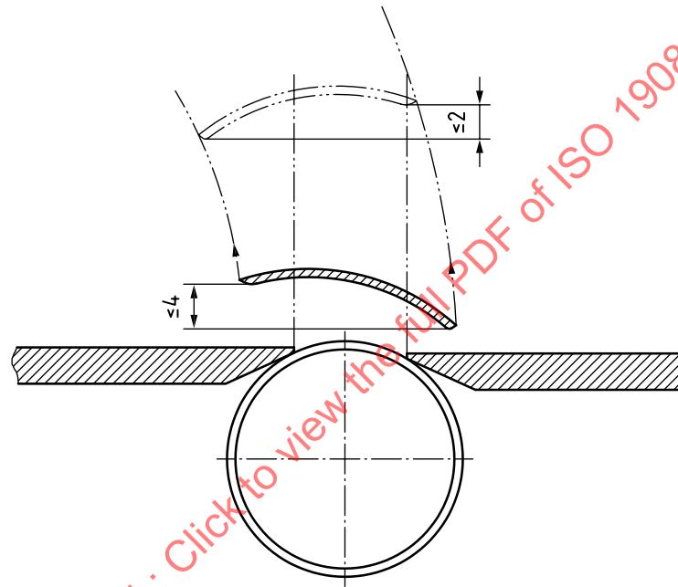
Figure 11 — Example of bridge-type guard
