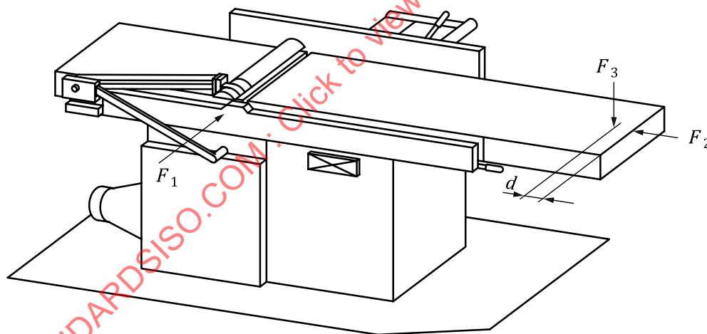
Figure C.1 — Stability test for displaceable machines (in surface planing setting)
