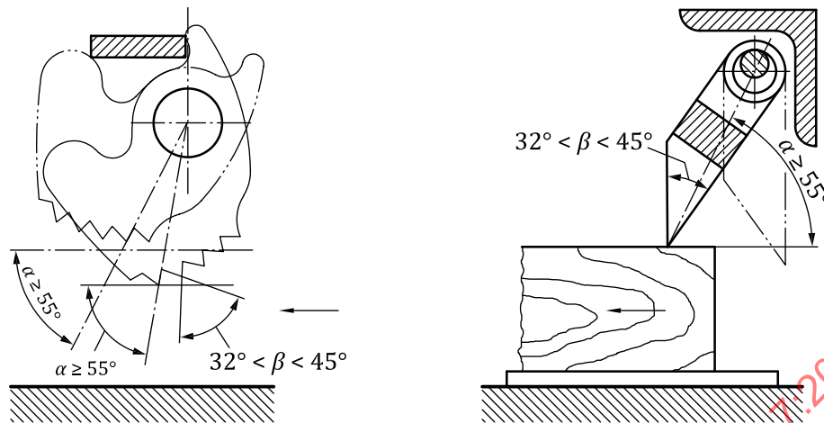
Figure 13 — Anti-kickback fingers (arrows indicate feed direction)
