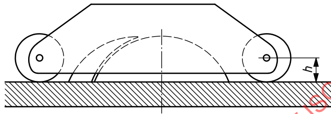
Figure 7 — Lead-in of saw blade guards mounted separately from the riving knife
