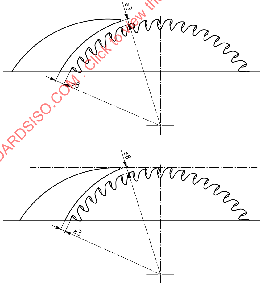
Figure 12 — Positioning limits for riving knife design
