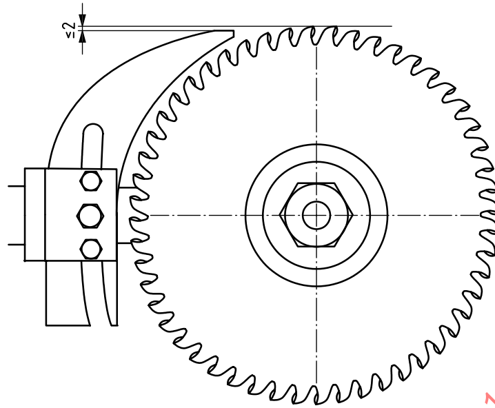
Figure 11 — Riving knife height adjustment
