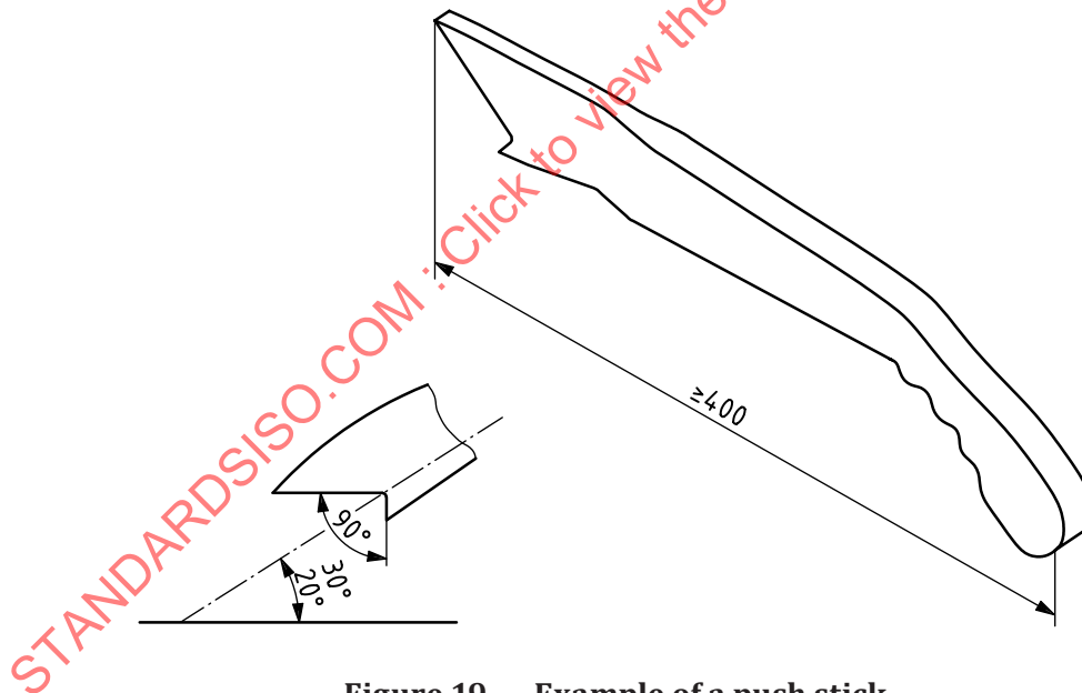
Figure 19 — Example of a push stick
