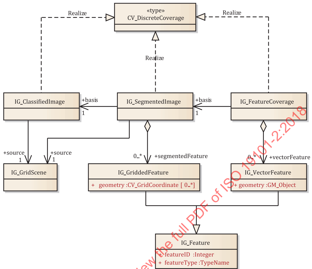
Figure 13 — Image classification and understanding class diagram
