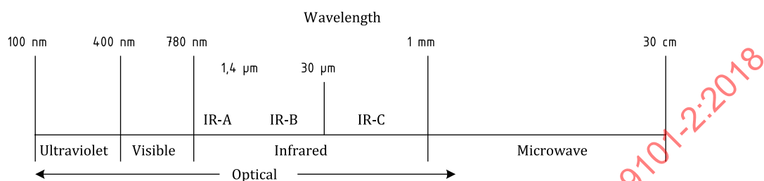
Figure 6 — Portion of the electromagnetic spectrum relevant for geographic imagery
