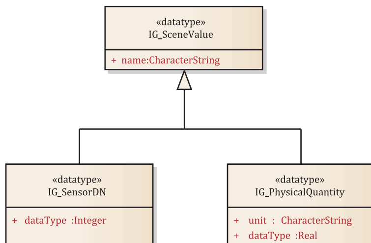
Figure 10 — IG_SceneValues
