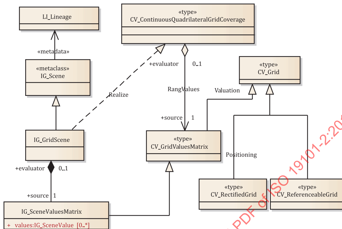
Figure 9 — IG_Scene
