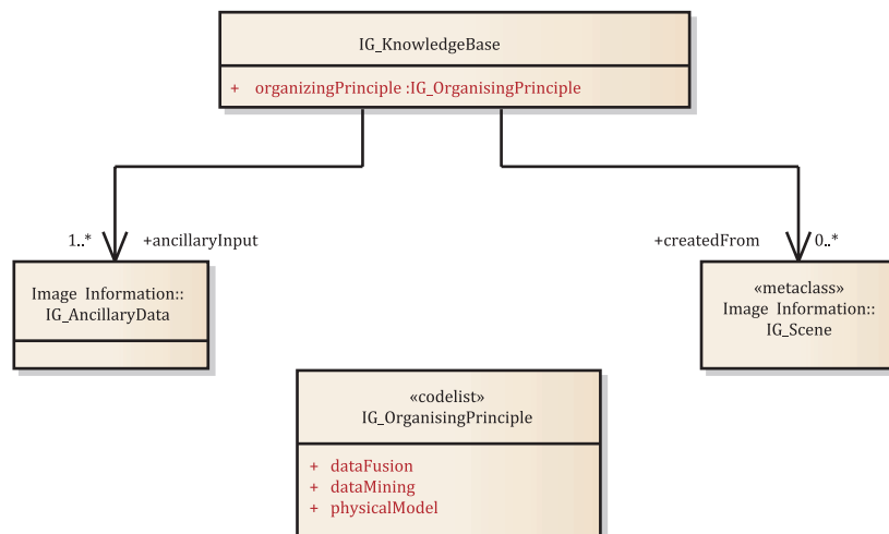
Figure 14 — IG_KnowledgeBase
