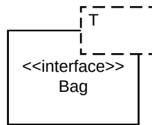
Figure 14 — Collection types — Bag type
