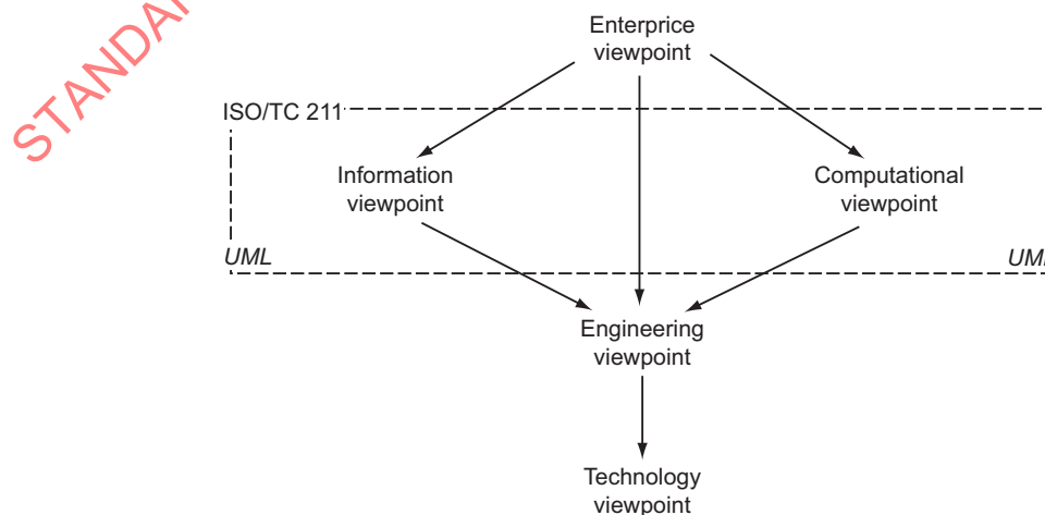
Figure E.8 — Viewpoints in the ISO RM-ODP model
