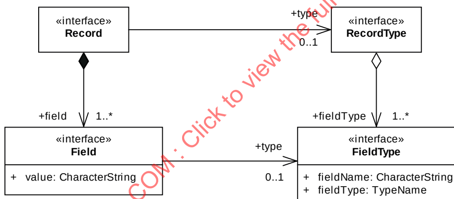
Figure 23 — Record and RecordType
