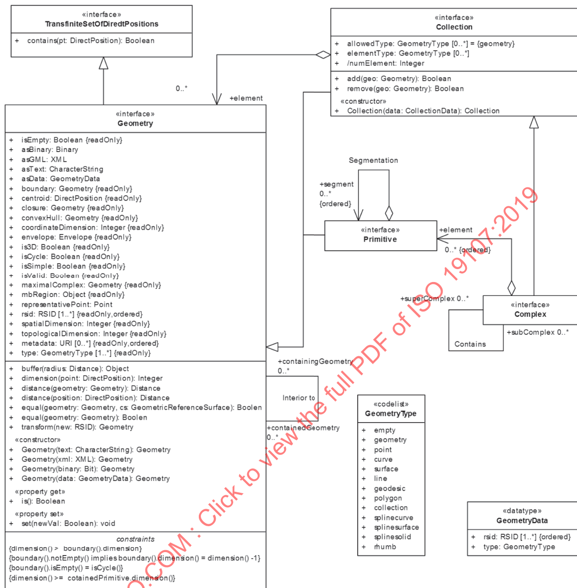
Figure 10 — Geometry root object
