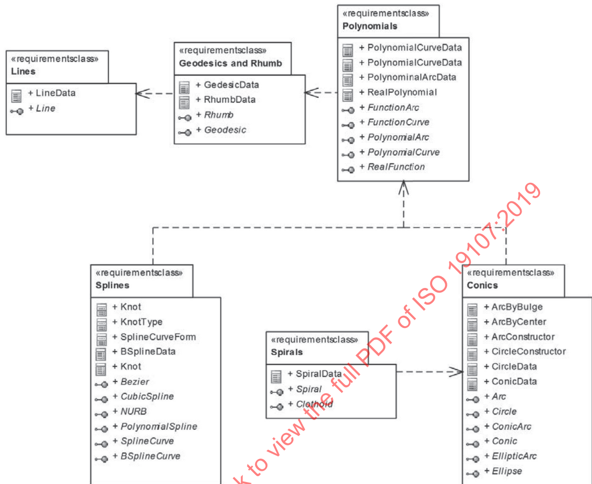
Figure 21 — Curve Packages and Requirements Classes
