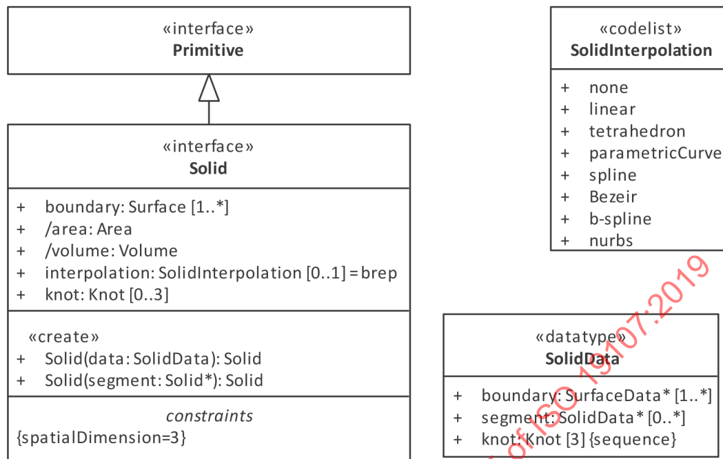
Figure 18 — Solid
