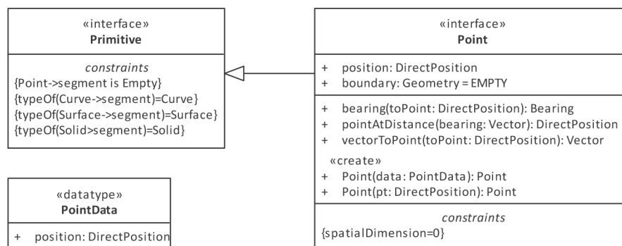
Figure 14 — Point
