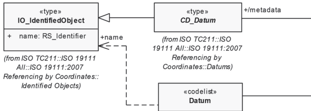
Figure 8 — Datum
