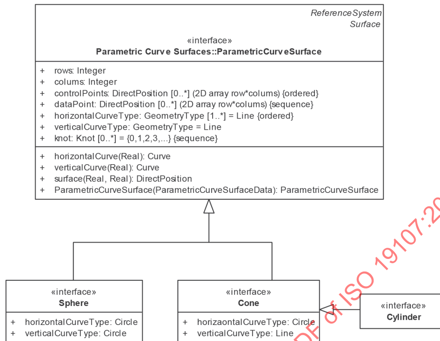
Figure 30 — Conics
