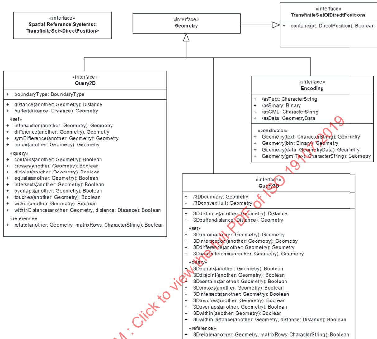
Figure 12 — Geometry Root Extensions
