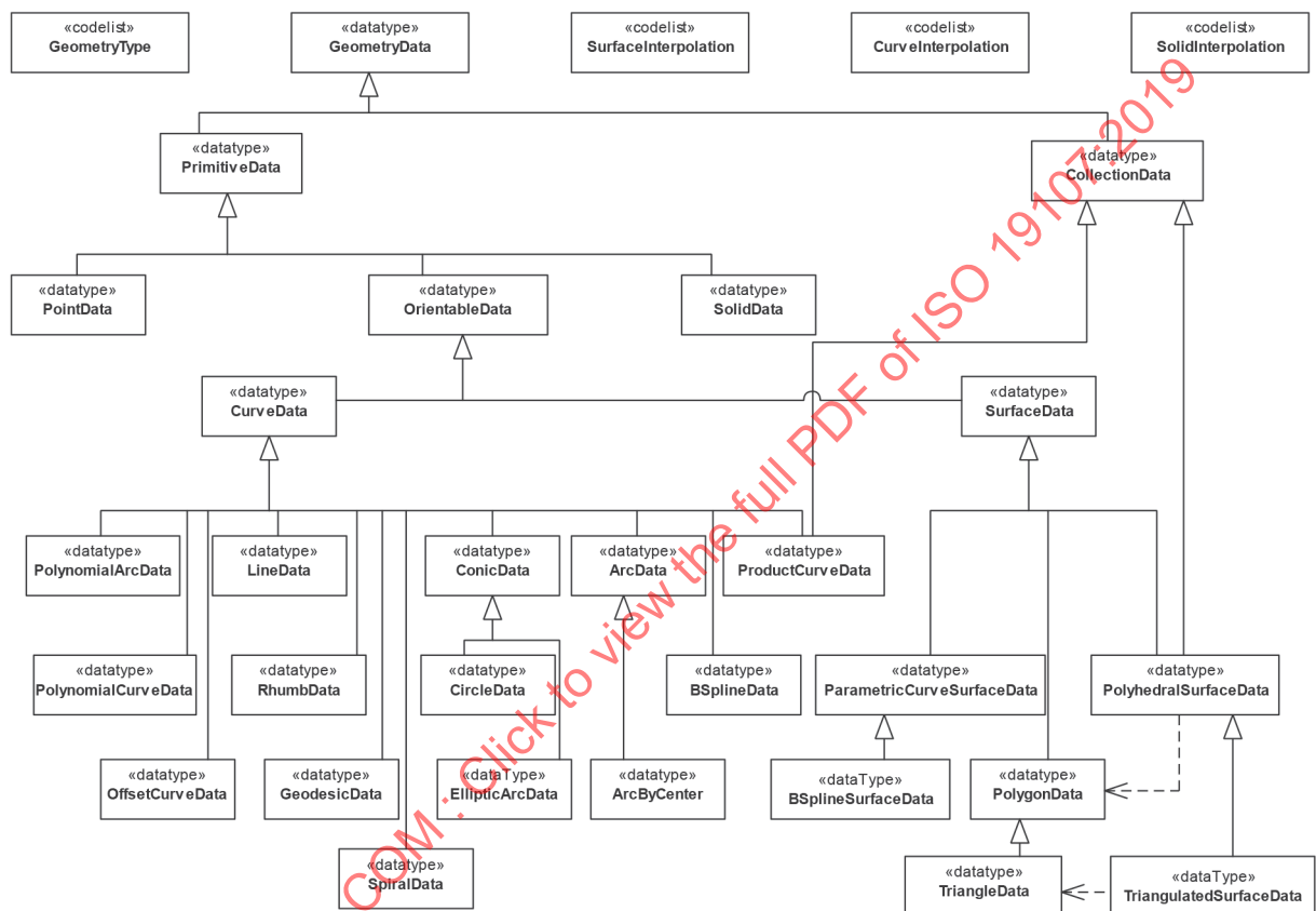
Figure 11 — Geometry Default Constructor Data Types
