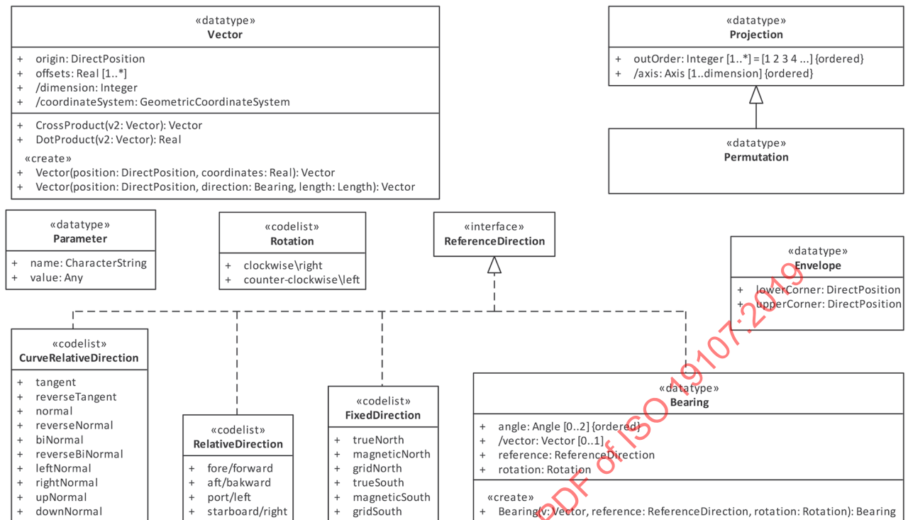
Figure 9 — Vector, Bearing and Permutation
