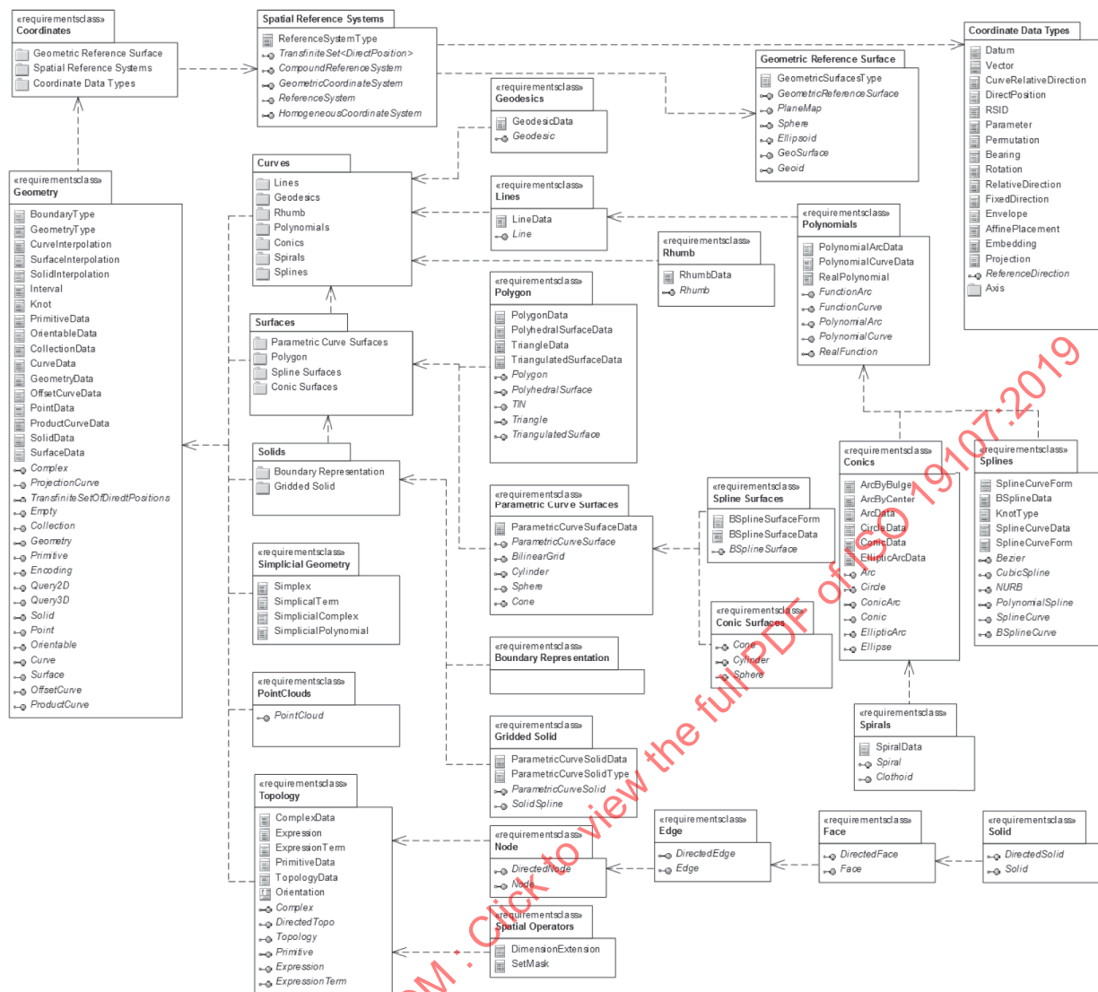
Figure 1 — Geometry packages and requirements classes
