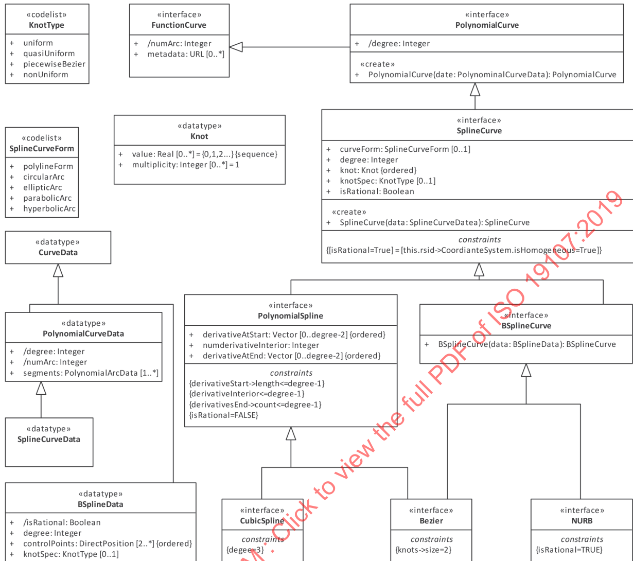
Figure 27 — Spline Curves
