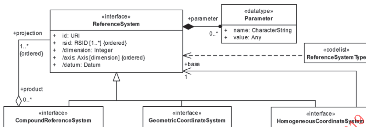
Figure 4 — Reference systems
