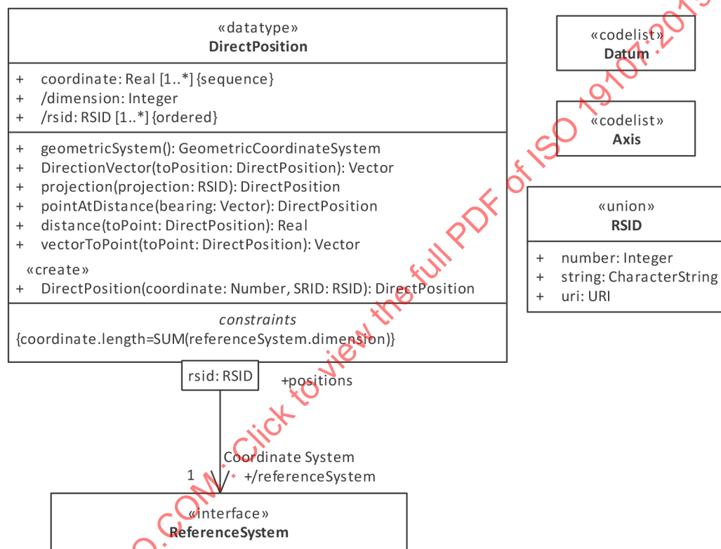
Figure 6 — DirectPosition
