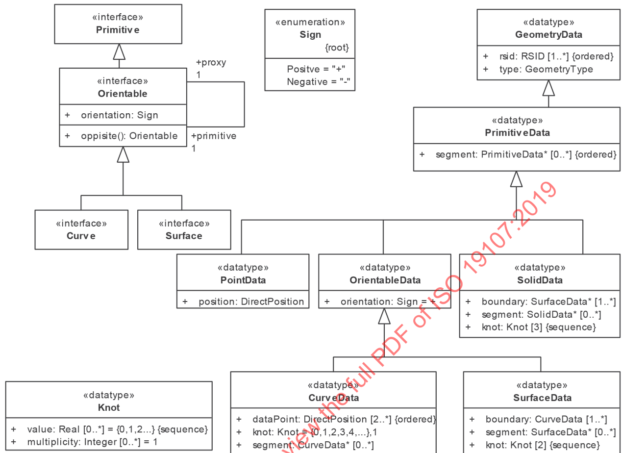
Figure 15 — Orientable Primitive
