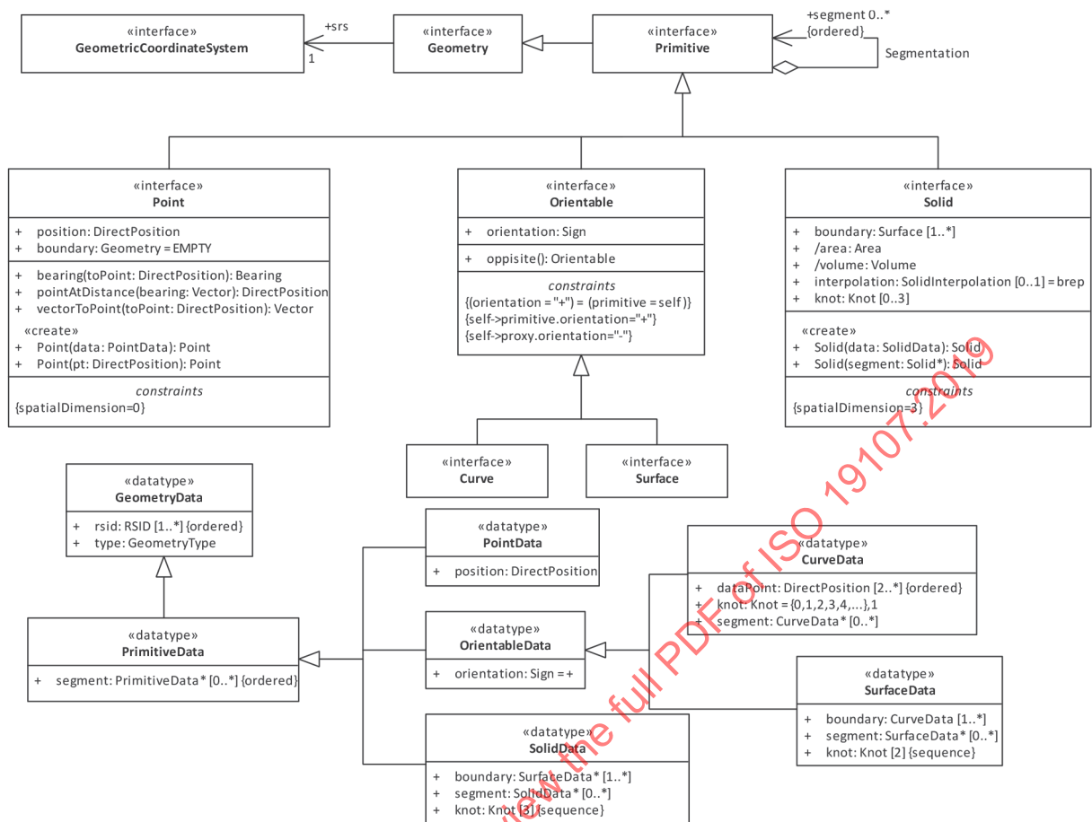
Figure 13 — Geometry Primitives and Their Default Constructors
