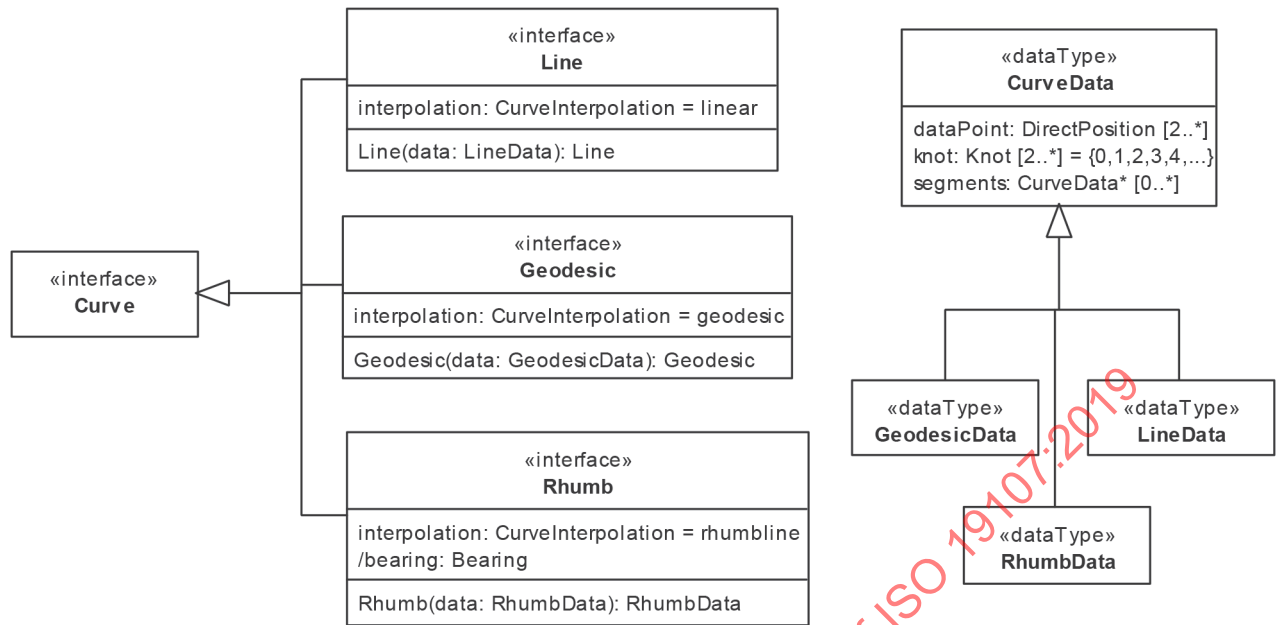
Figure 23 — Line, geodesic and rhumb curves
