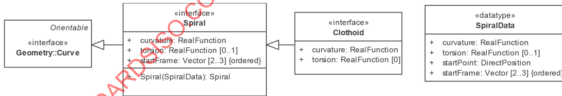
Figure 26 — Spirals
