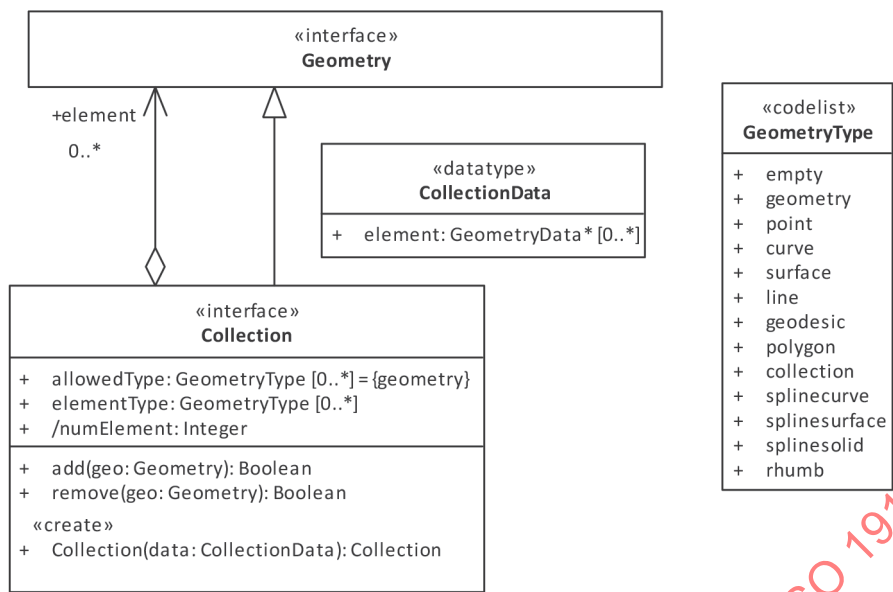
Figure 19 — Geometry Collection
