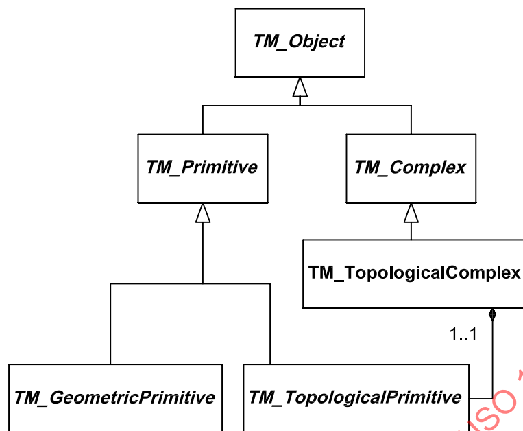
Figure 2 — Temporal objects
