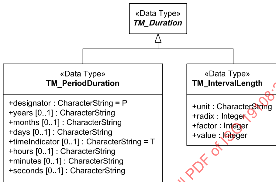
Figure 5 — TM_Duration
