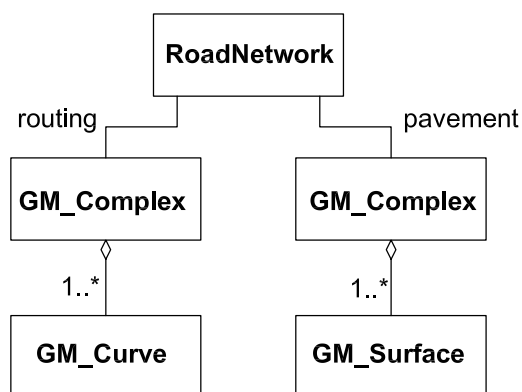
Figure 31 — Example of independent spatial complexes
