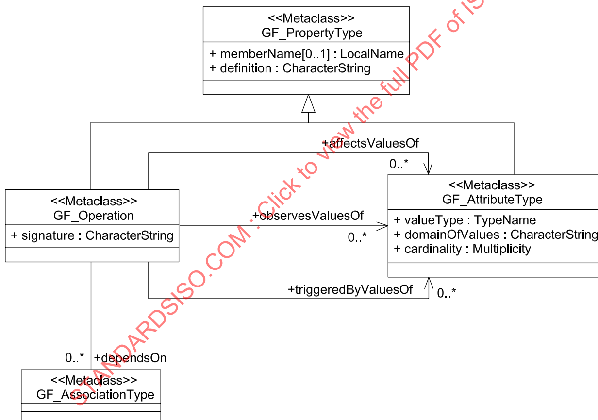
Figure 8 — Behaviour of feature types
