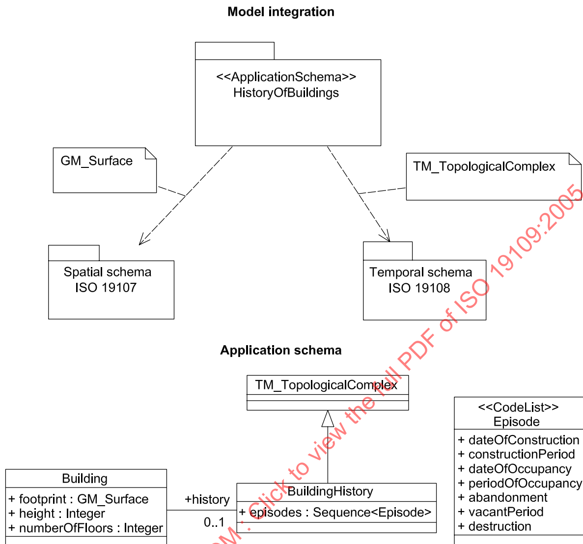
Figure 18 — Example of TM_TopologicalComplex used as a temporal feature attribute
