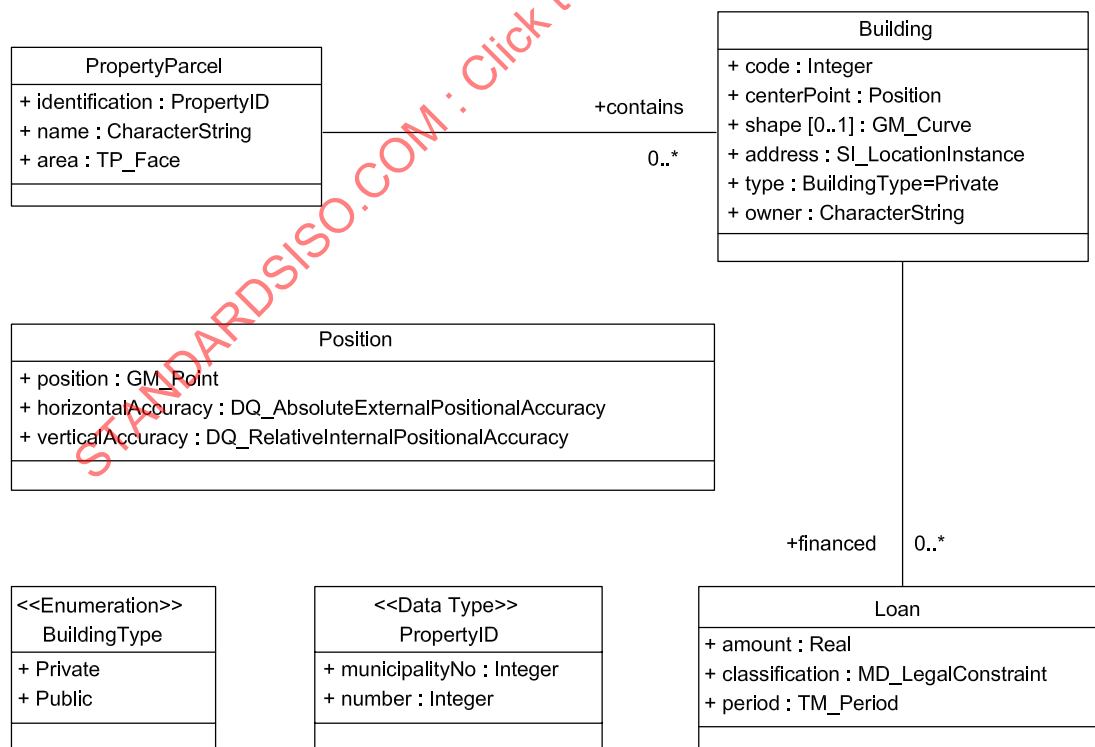
Figure 11 — Example of UML implementation of feature types
