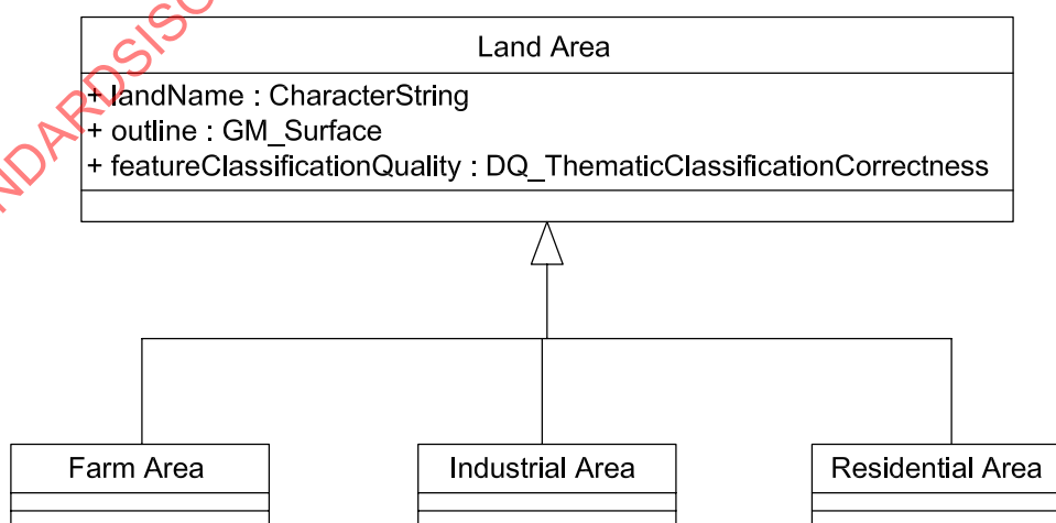
Figure 14 — Example of quality of features instances
