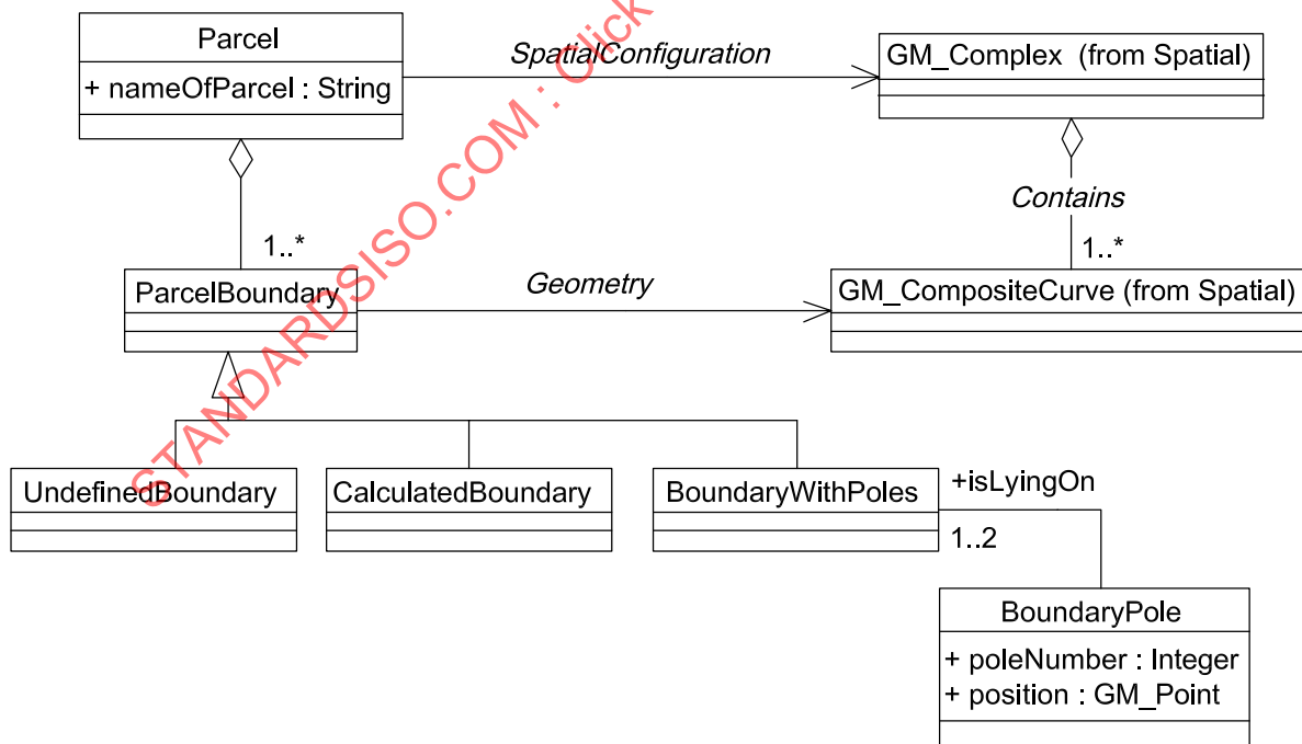
Figure 24 — Example of spatial complex defined in application schema
