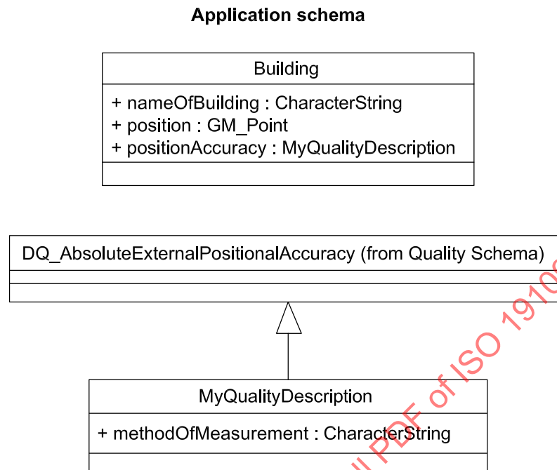
Figure 16 — Example of user-defined quality
