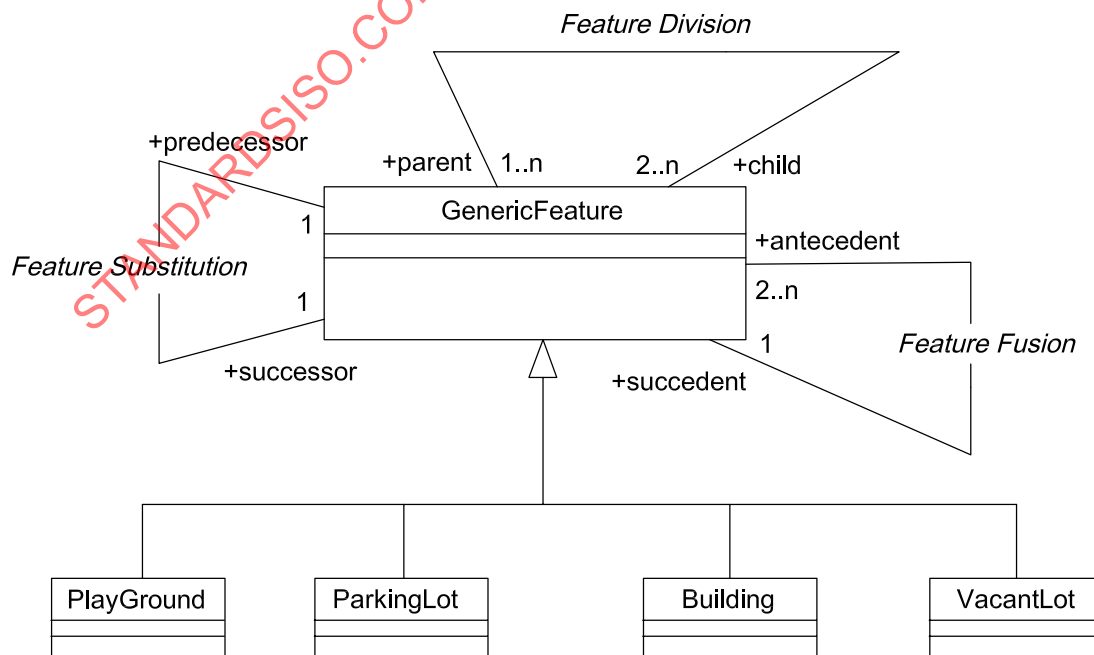
Figure 21 — Example of feature succession at the generic feature level
