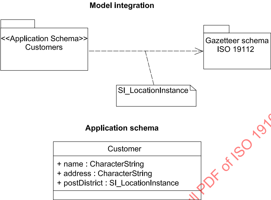
Figure 34 — Example of spatial referencing by geographic identifier
