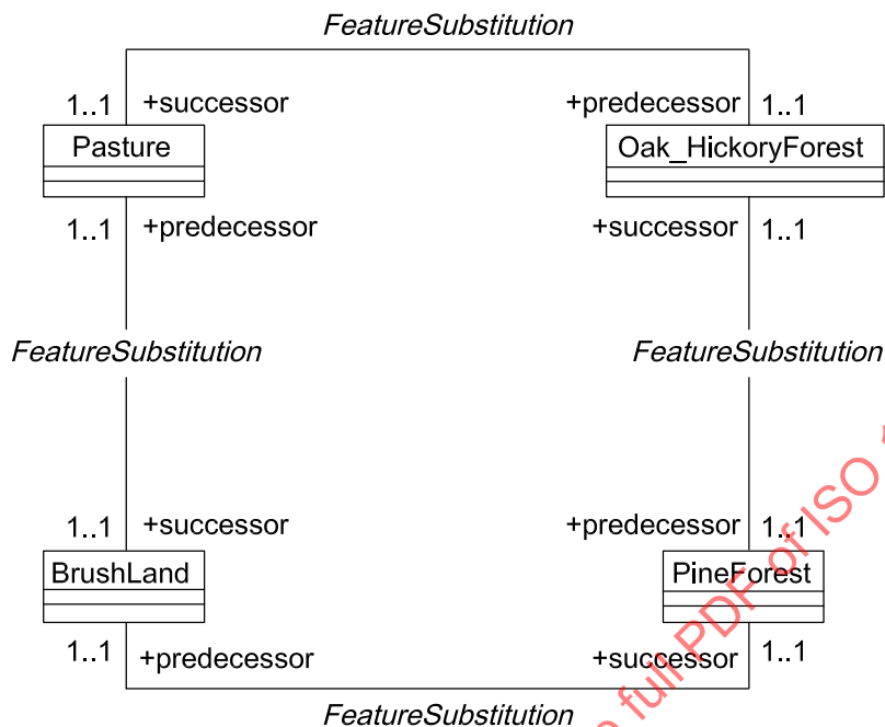
Figure 20 — Example of feature succession between feature types
