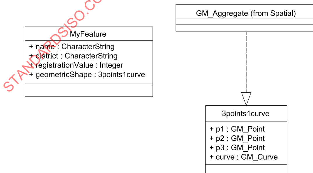
Figure 23 — Example of spatial aggregate defined in application schema
