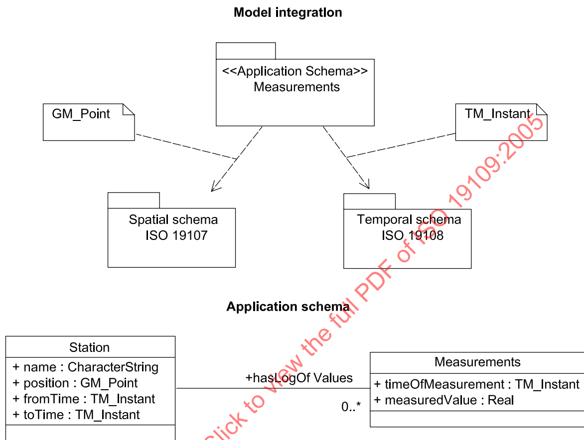
Figure 17 — Example of temporal attribute
