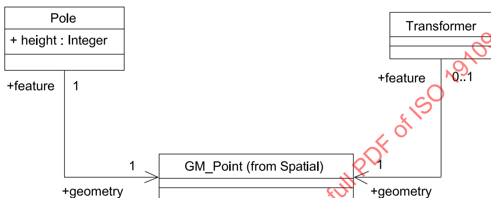
Figure 28 — Example of features sharing geometry
