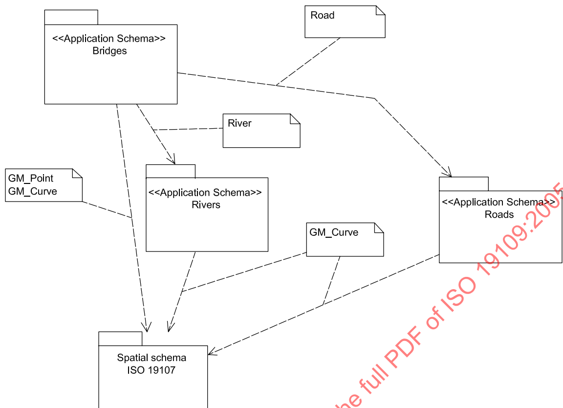
Figure 10 — Example of an application schema based on other application schemas
