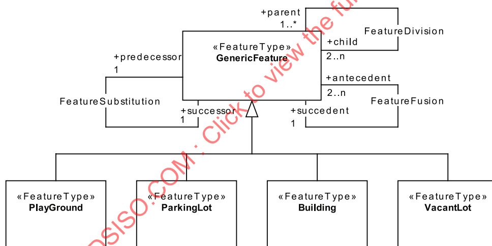
Figure 23 — Example of feature succession at the generic feature level
