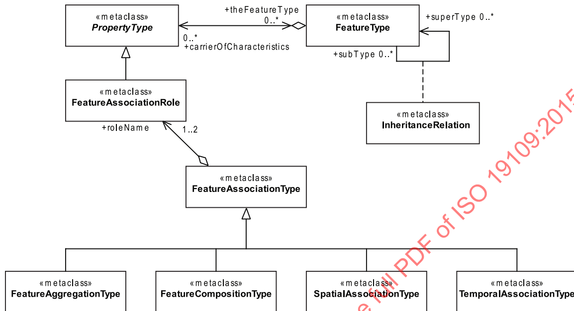
Figure 8 — Relationships between feature types
