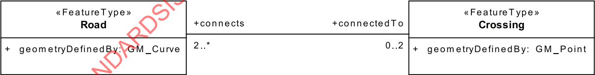
Figure 29 — Example of spatial associations implemented as associations in the application schema
