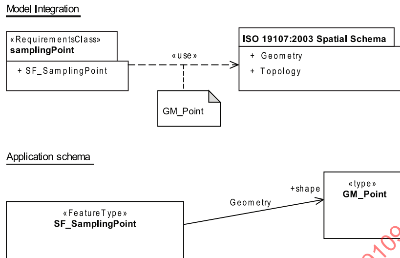
Figure 24 — Example of spatial attributes in UML
