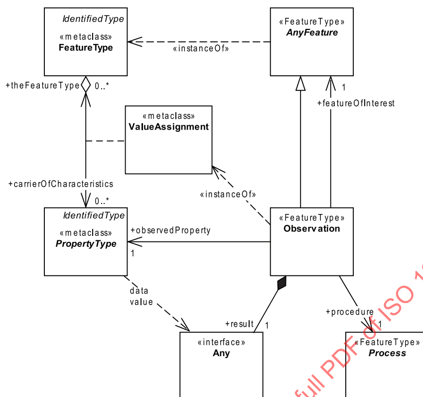
Figure 36 — Key elements of the observation schema (ISO 19156) related to General Feature Model (Clause 7)
