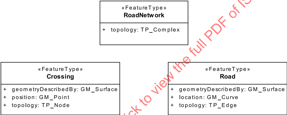
Figure 28 — Example of spatial associations implemented by use of spatial objects
