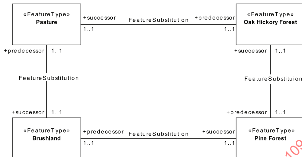
Figure 22 — Example of feature succession between feature types
