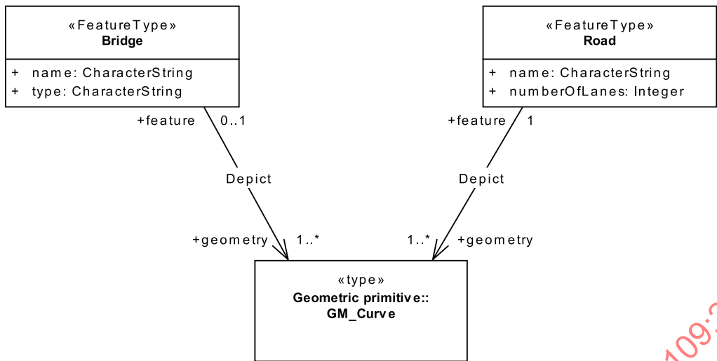
Figure 31 — Example of partial sharing of geometry between features
