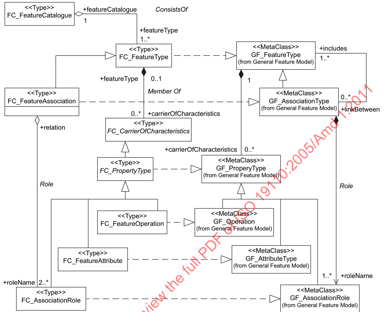
Figure B.3 — Derivation FC_FeatureType , FC_FeatureAttribute , FC_FeatureAssociation , and FC_AssociationRole from general feature model metaclasses
