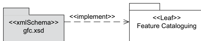
Figure E.2 — Organization of the gfc namespace
