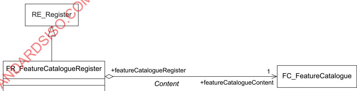
Figure F.1 — Feature catalogue register as a subclass of RE_Register
