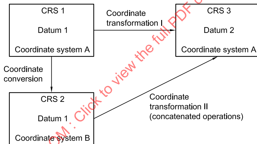
Figure D.1 — Coordinate conversion and coordinate transformation
