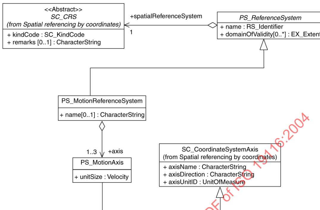
Figure 12 — UML depiction of PS_MotionReferenceSystem class with its attributes and associations
