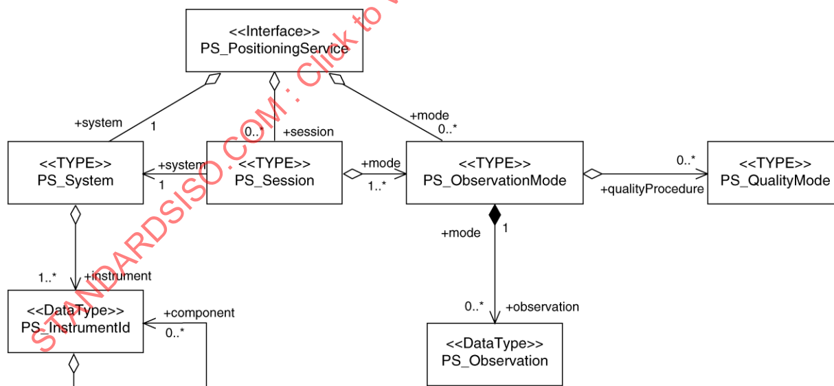
Figure 5 — UML depiction of the major data classes of positioning services
