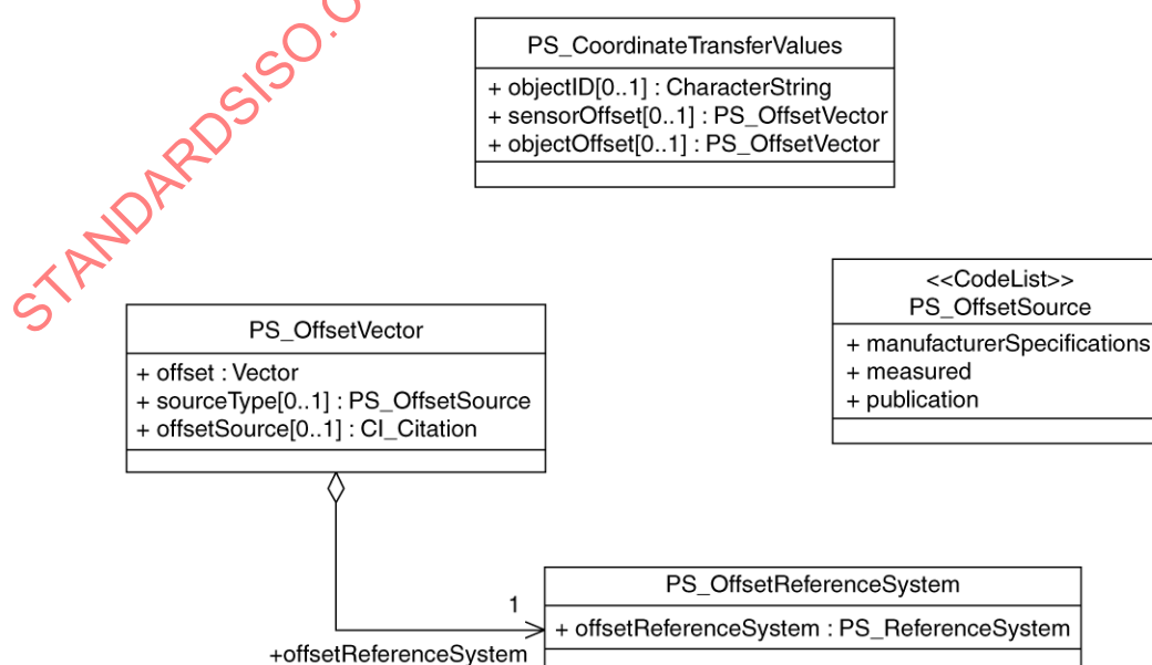
Figure 16 — UML depiction of PS_CoordinateTransferValues class with its attributes and associations
