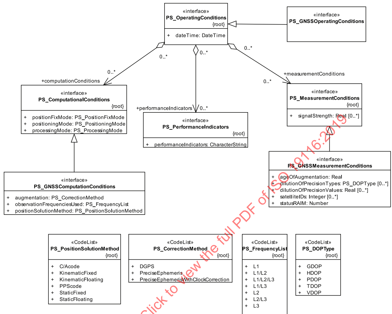
Figure D.1 — UML diagram — PS_GNSSOperatingConditions class
