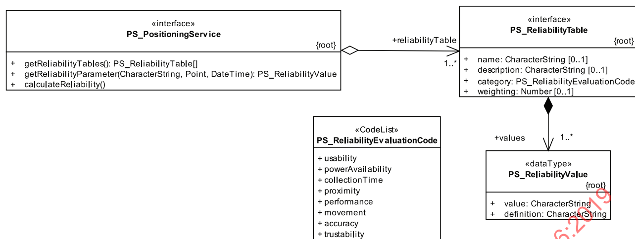
Figure 12 — UML diagram — Reliability model
