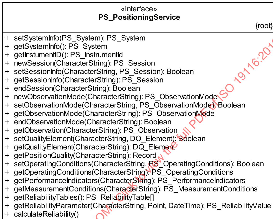
Figure 11 — UML diagram — Operations of positioning services
