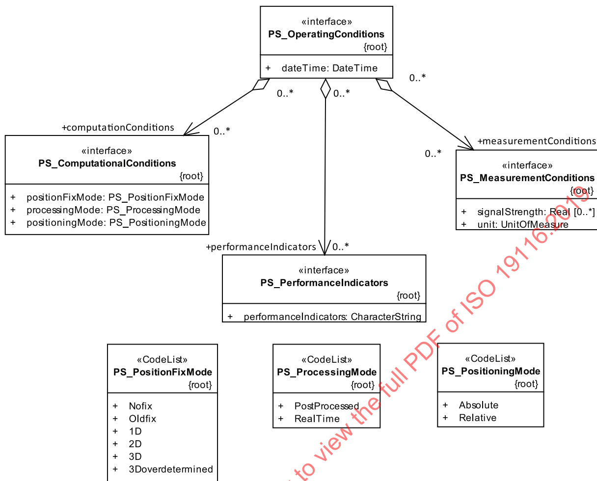
Figure 13 — UML diagram — Technology specific operation conditions
