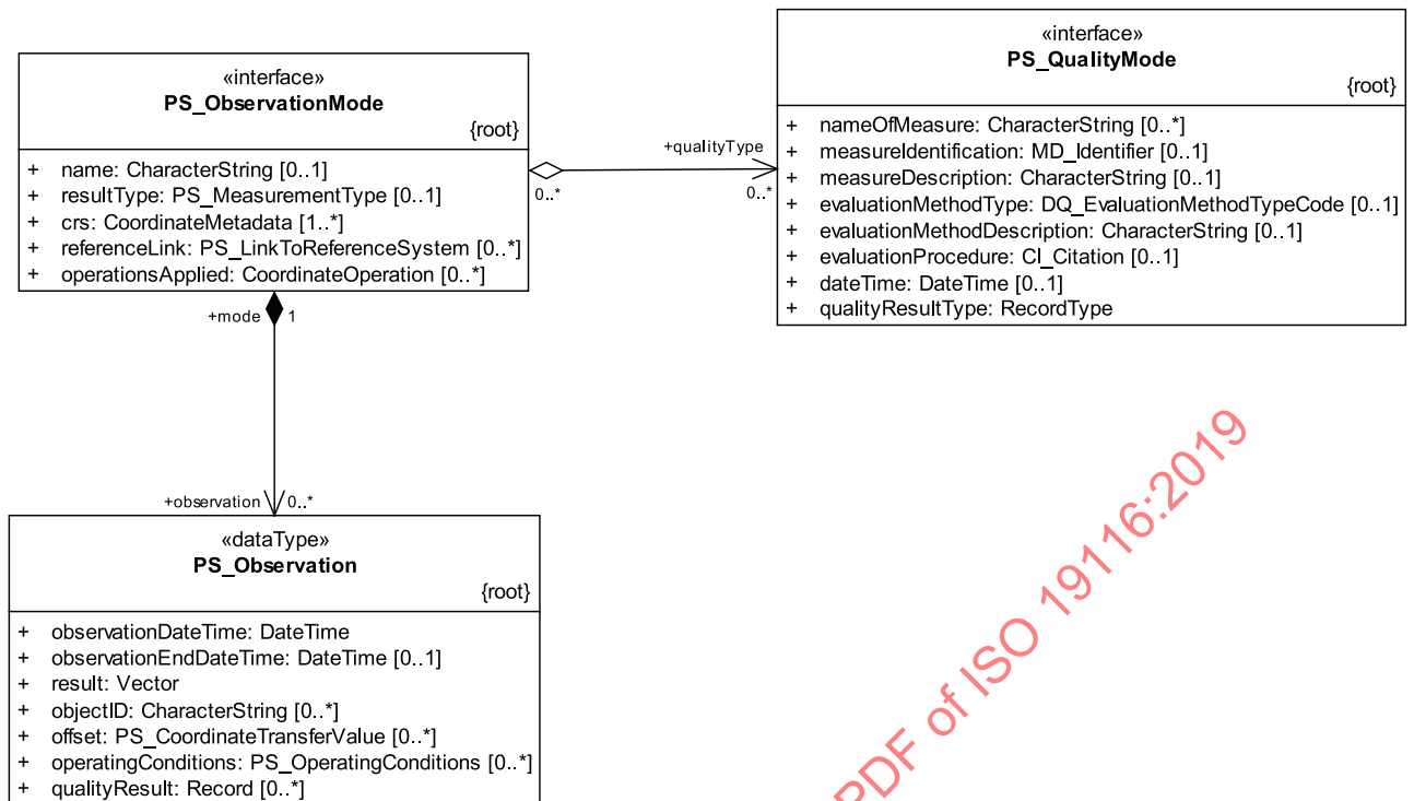
Figure 10 — UML diagram — Positioning services quality reporting classes
