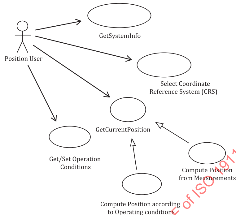
Figure C.1 — Use case for obtaining coordinates from a positioning service
