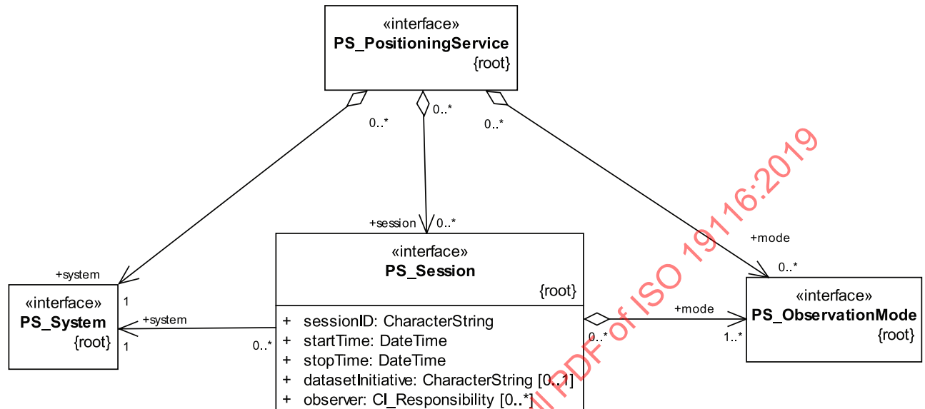
Figure 5 — UML diagram — PS_Session class
