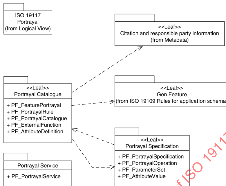
Figure 5 — Portrayal information and portrayal service
