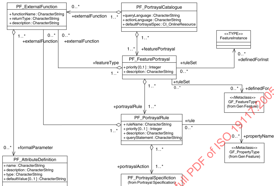
Figure 7 — Portrayal catalogue package
