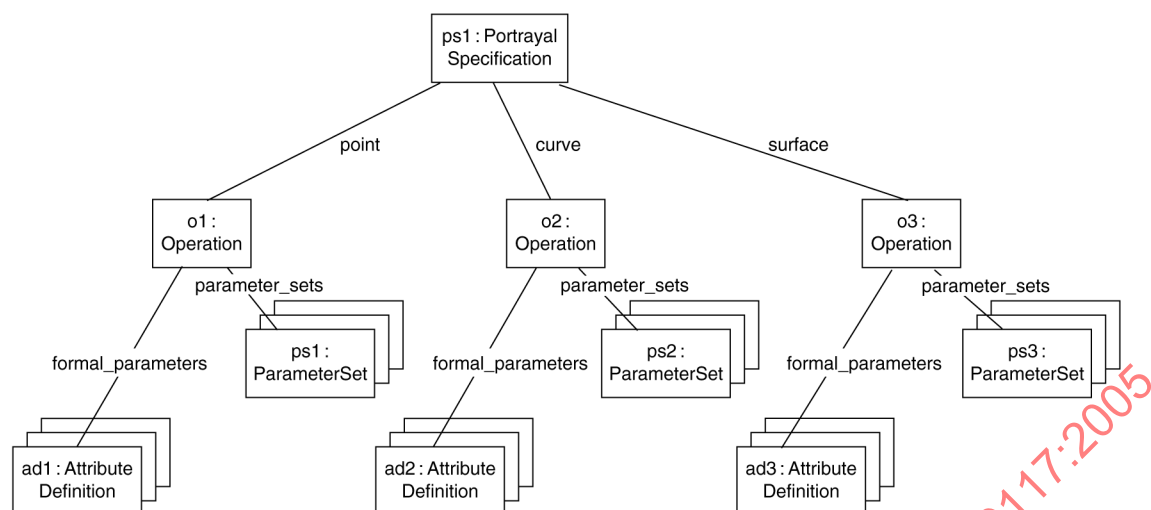
Figure B.1 — Object diagram showing a subset of example 2
