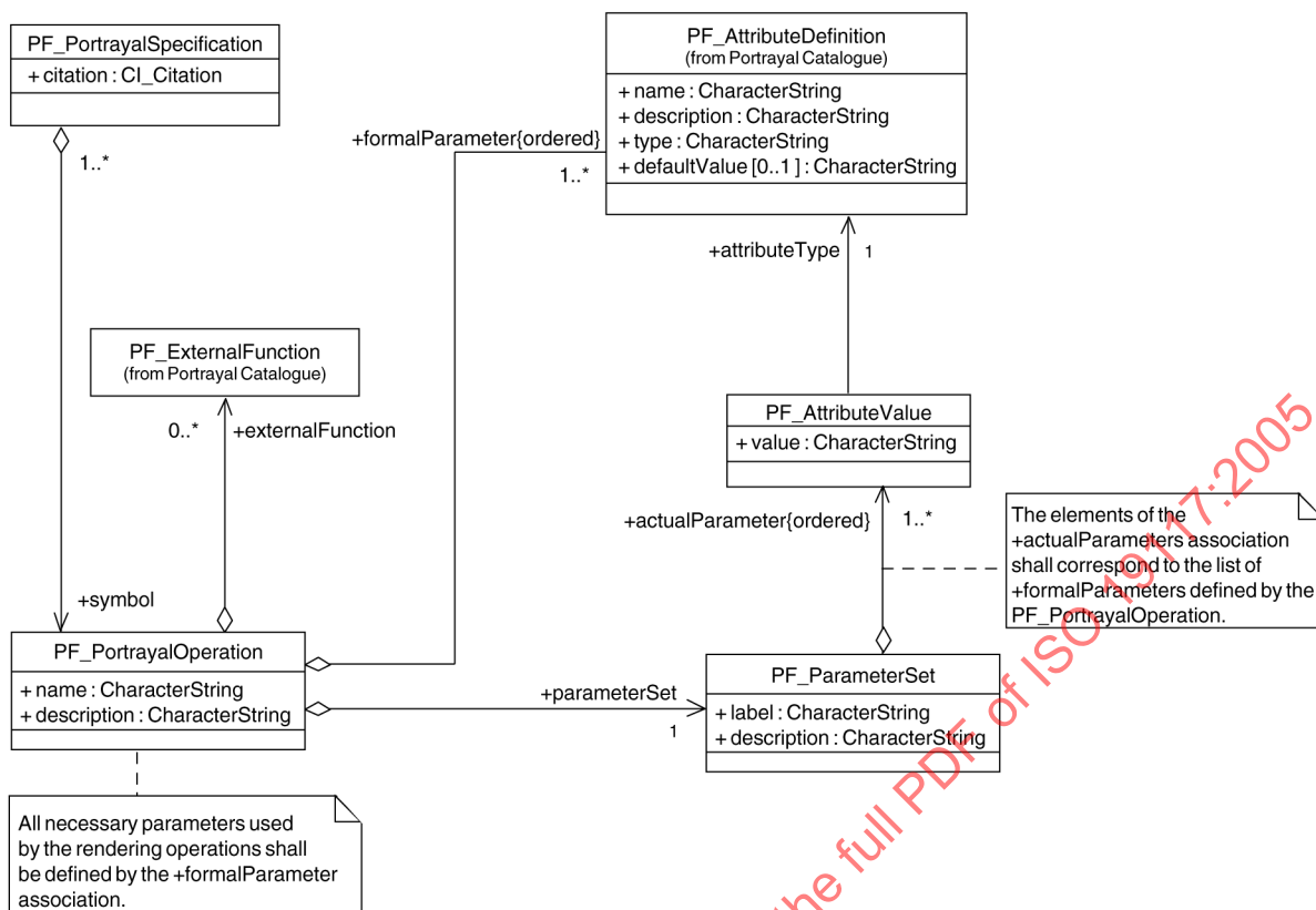
Figure 8 — Portrayal specification package
