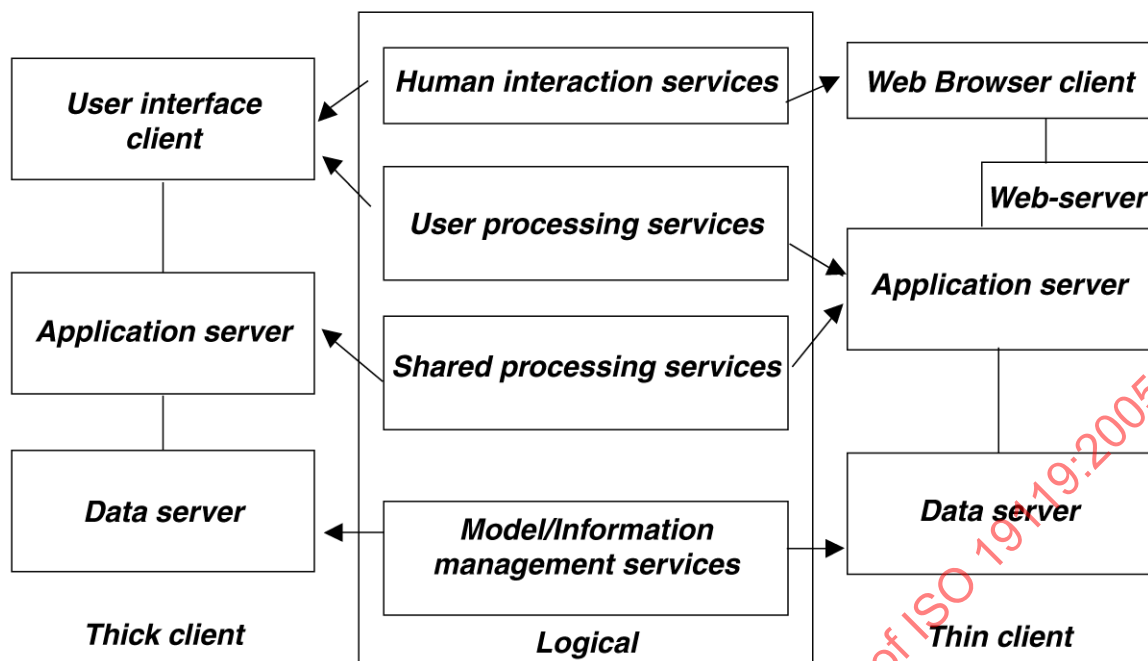
Figure 12 — Mapping logical four-tier to thick and thin clients
