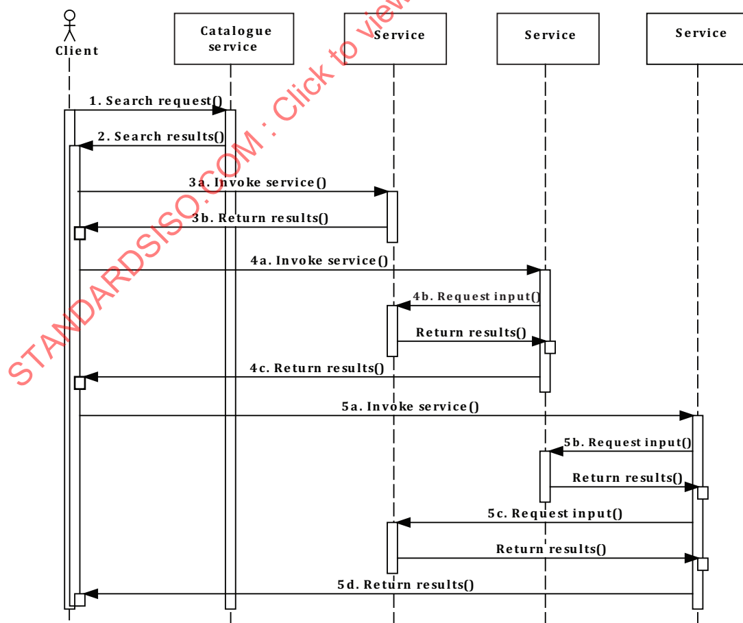
Figure 8 — Transparent chaining — User-defined chaining architecture pattern
