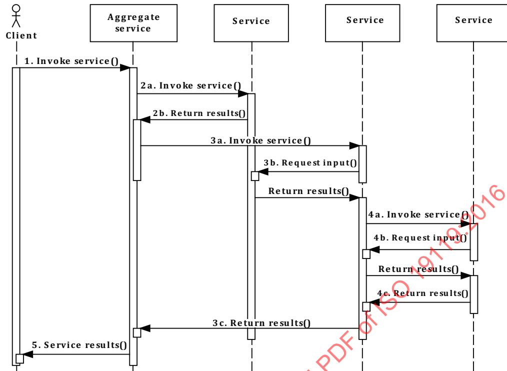
Figure 10 — Opaque chaining
