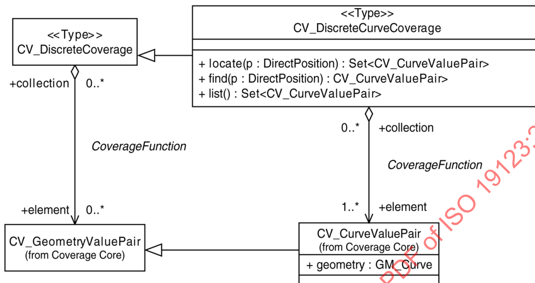
Figure 8 — CV_DiscreteCurveCoverage
