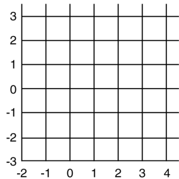
Figure 13 — Example — A 7 × 7 two-dimensional orthogonal grid
