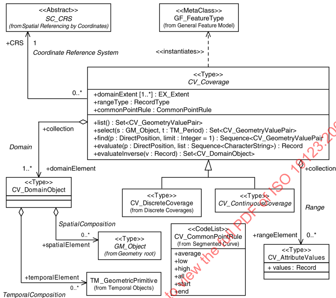
Figure 2 — CV_Coverage
