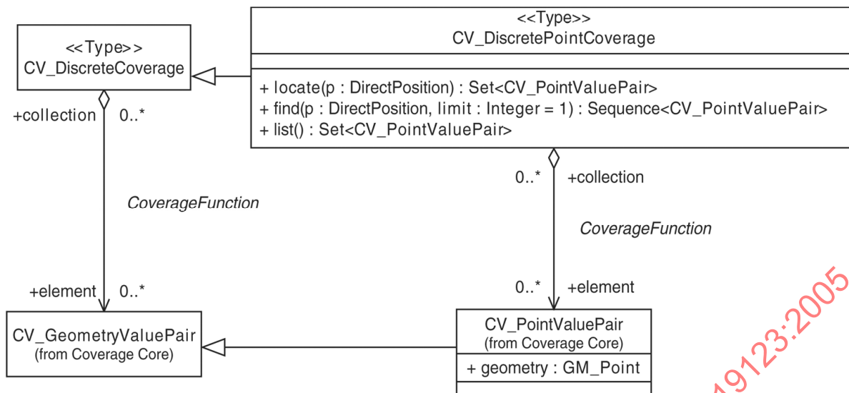
Figure 6 — CV_DiscretePointCoverage
