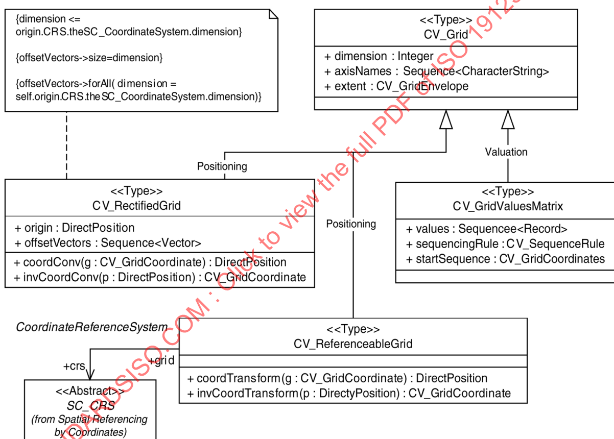
Figure 17 — CV_Grid subclasses
