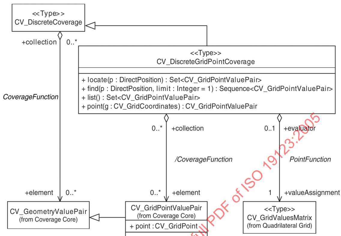
Figure 7 — CV_DiscreteGridPointCoverage
