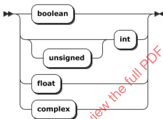
Figure C.16 — rangeType
