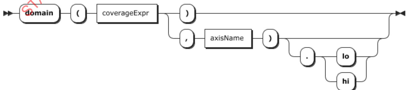
Figure C.22 — getDomainExpr
