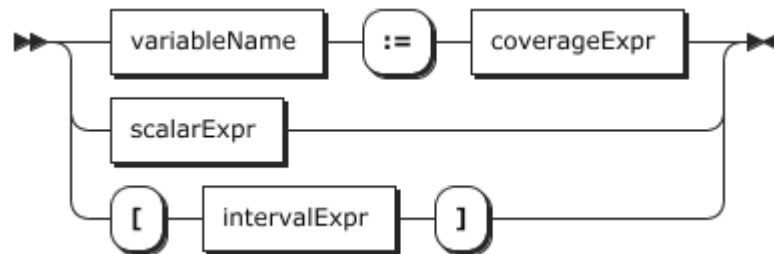
Figure C.3 — letBinding
