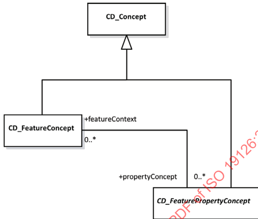
Figure 5 — CD_FeatureConcept
