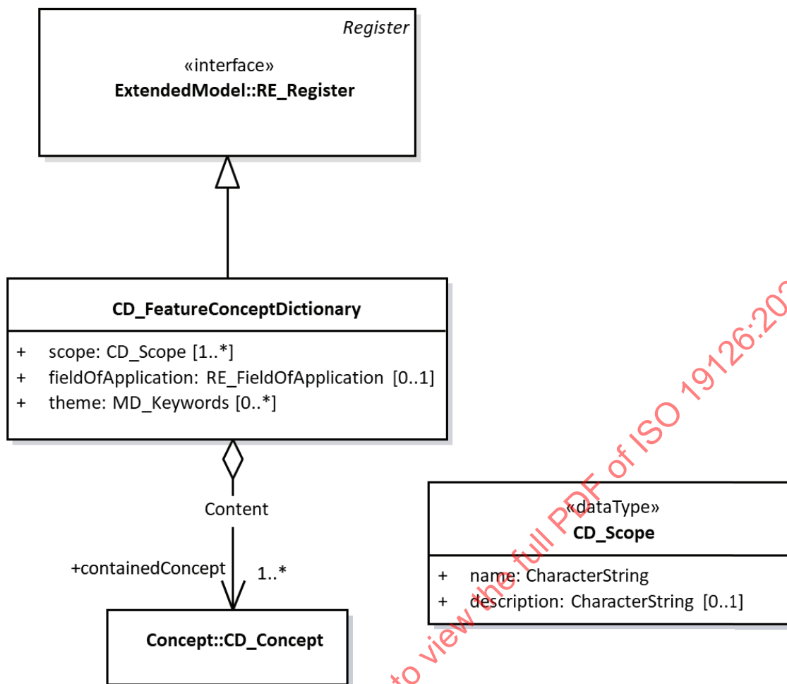
Figure 3 — CD_FeatureConceptDictionary
