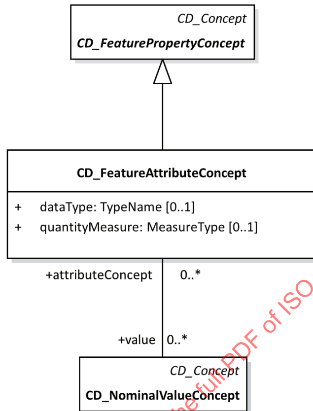
Figure 6 — CD_FeatureAttributeConcept
