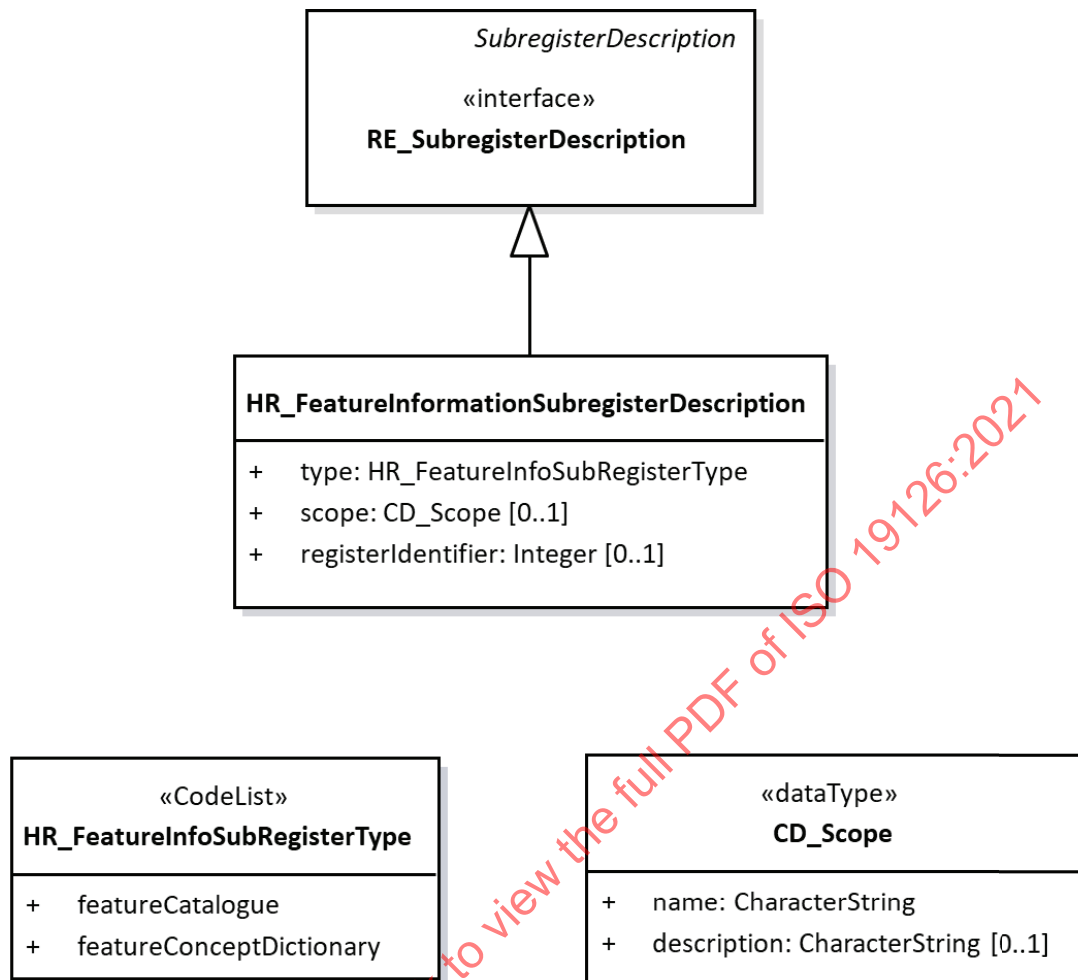
Figure 10 — HR_FeatureInformationSubregisterDescription
