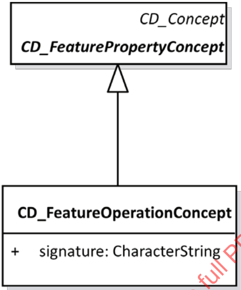
Figure 9 — CD_FeatureOperationConcept
