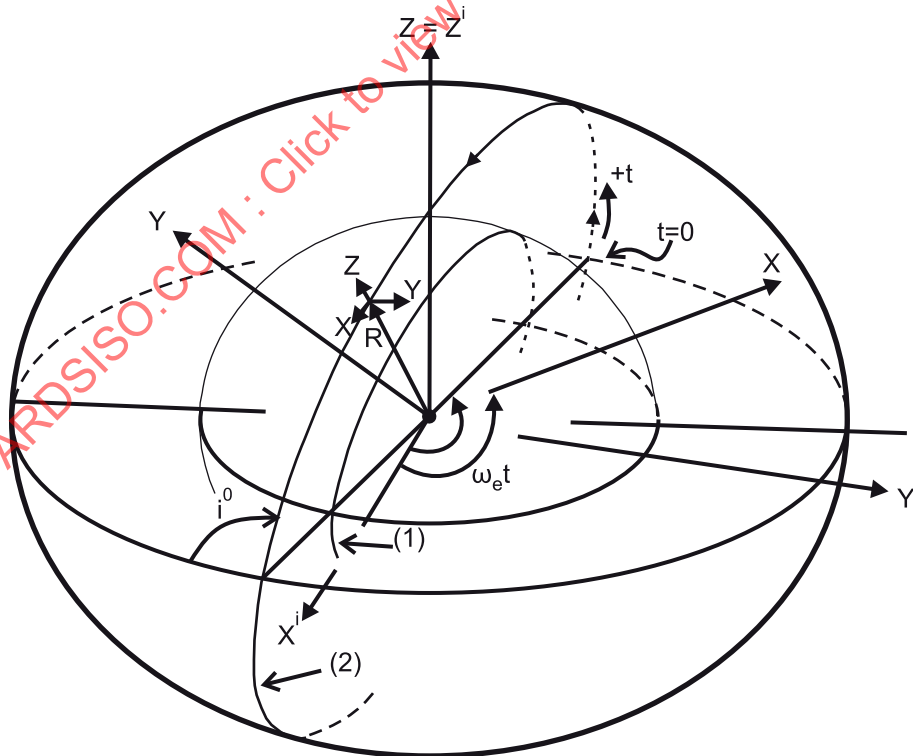
Figure C.5 — Orbital geometry
