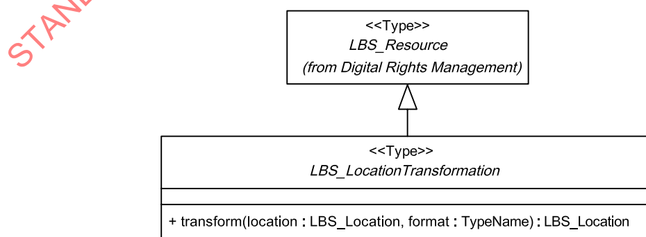
Figure 20 — Context Diagram: LBS_LocationTransformation
