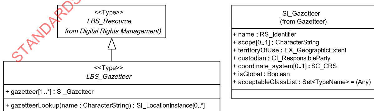
Figure 23 — Context Diagram: LBS_Gazetteer
