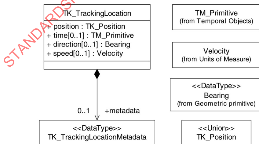
Figure 4 — Context Diagram: TK_TrackingLocation
