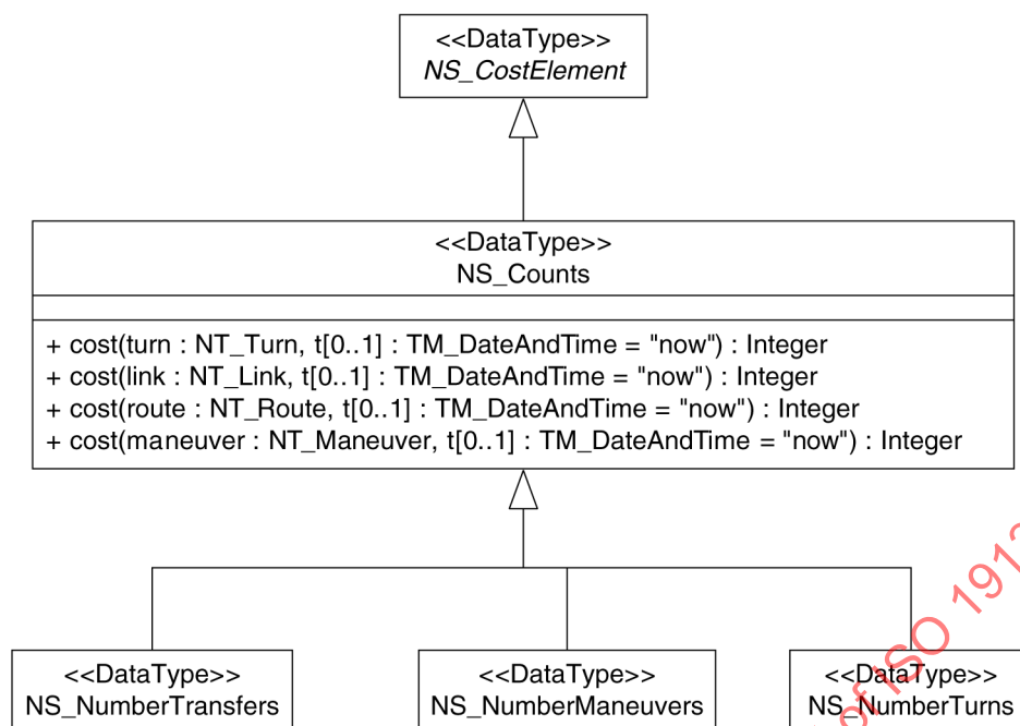
Figure 61 — Context Diagram: NS_Counts
