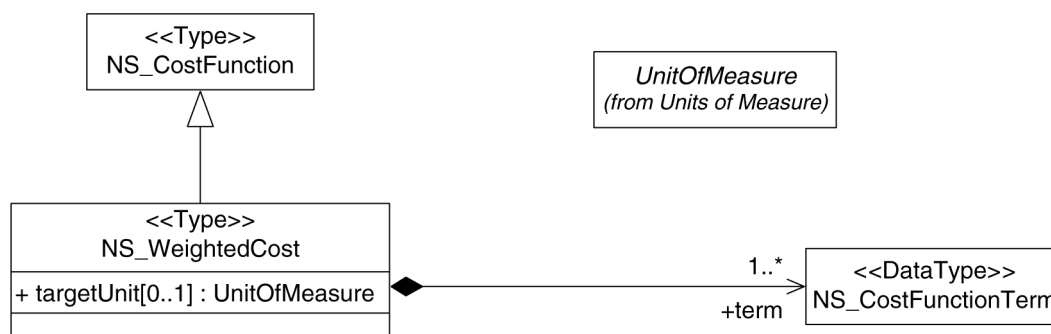
Figure 66 — Context Diagram: NS_WeightedCost
