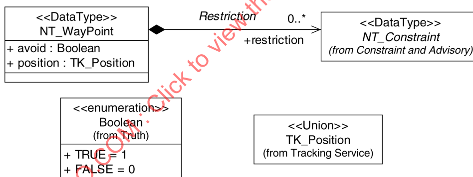
Figure 91 — Context Diagram: NT_WayPoint
