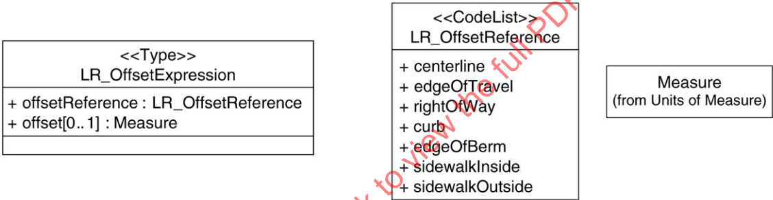
Figure 36— Context Diagram: LR_OffsetExpression
