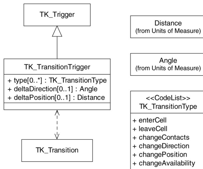
Figure 10 — Context Diagram: TK_TransitionTrigger
