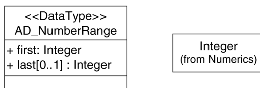
Figure 88 — Context Diagram: AD_NumberRange
