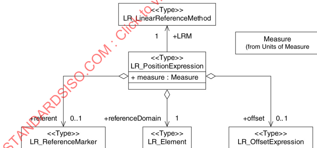
Figure 30 — Context Diagram: LR_PositionExpression
