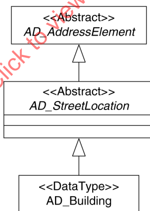
Figure 80 — Context Diagram: AD_StreetLocation
