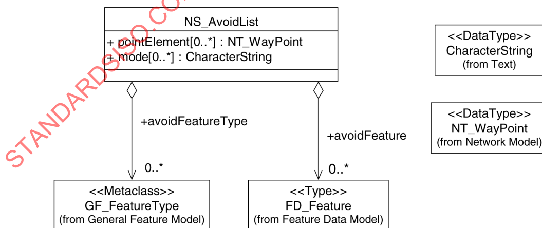
Figure 69 — Context Diagram: NS_AvoidList
