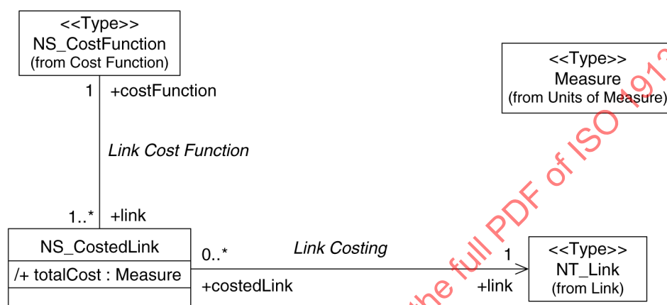
Figure 50 — Context Diagram: NS_CostedLink
