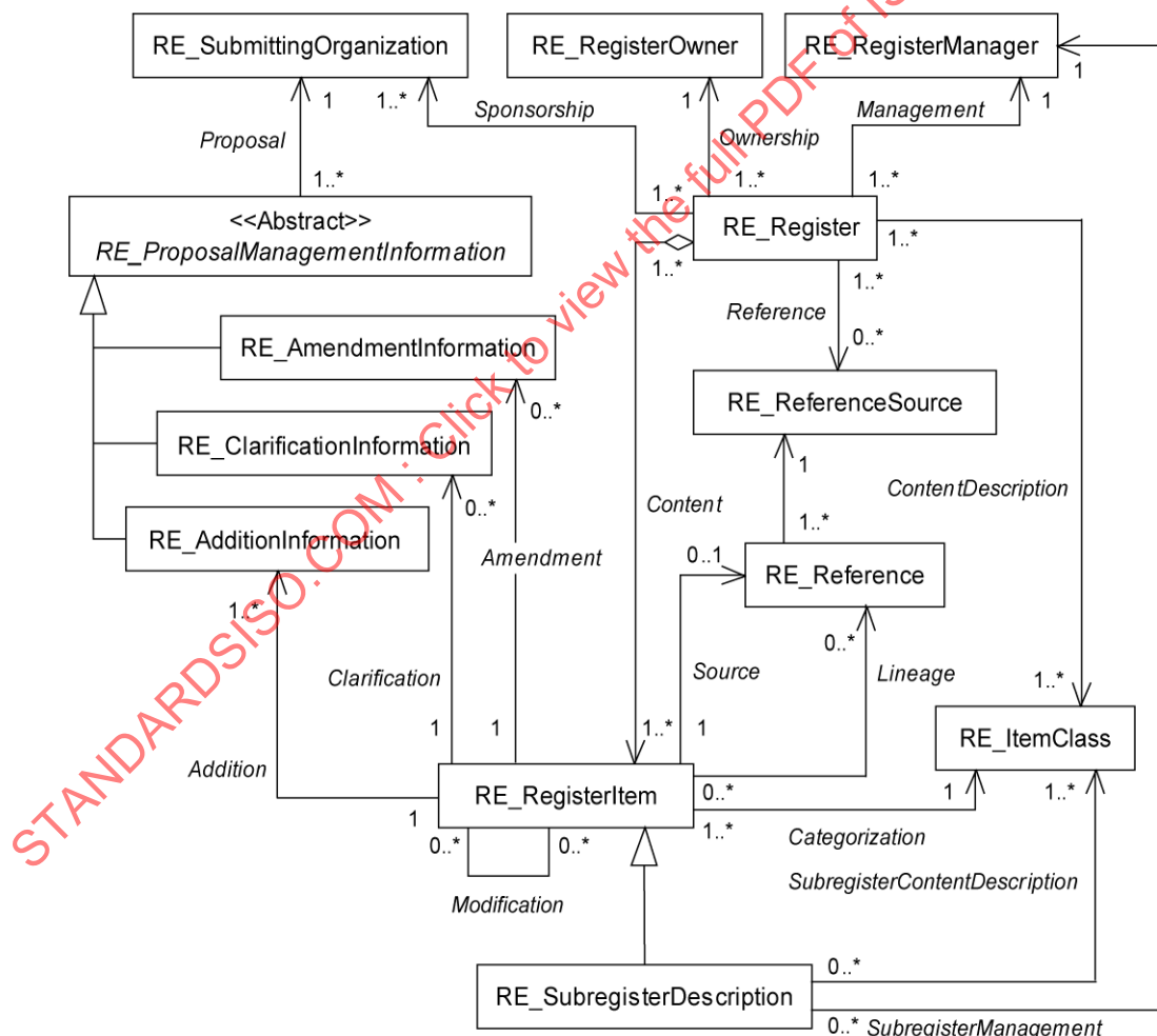
Figure 7 — The register schema
