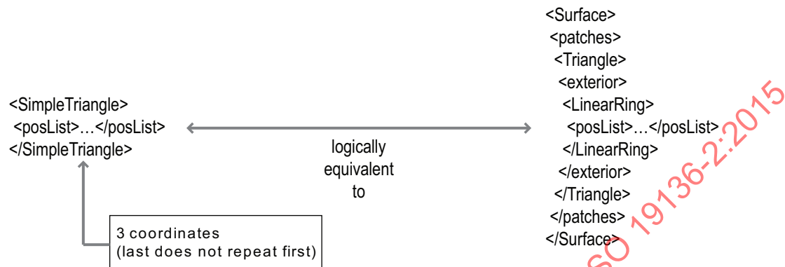
Figure 4 — SimpleTriangle encoding
