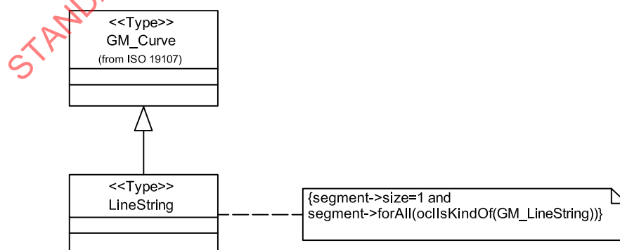
Figure D.46 — GM_Curve with a single GM_LineString segment
