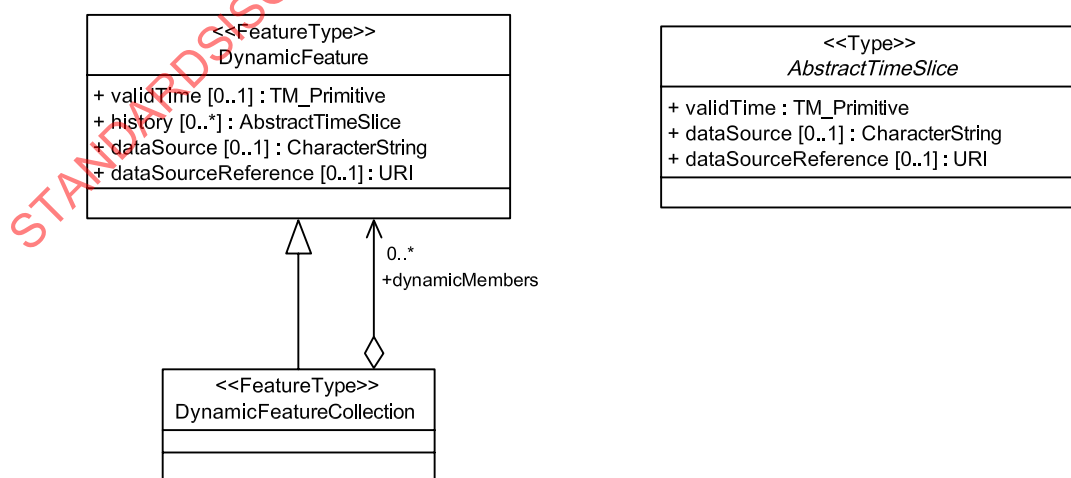
Figure D.56 — Dynamic features
