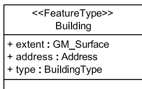
Figure E.2 — A feature type &lt;informative&gt;
