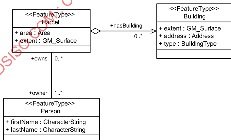
Figure E.6 — Associations <informative>
