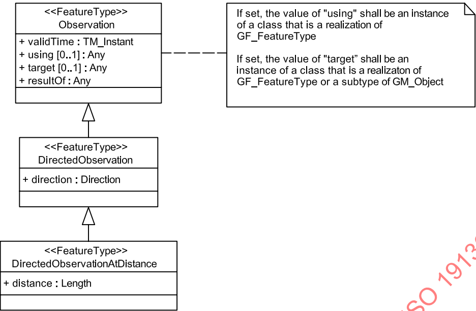
Figure D.66 — Observation
