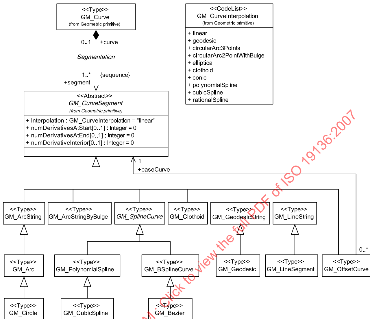
Figure D.15 — Curve segments
