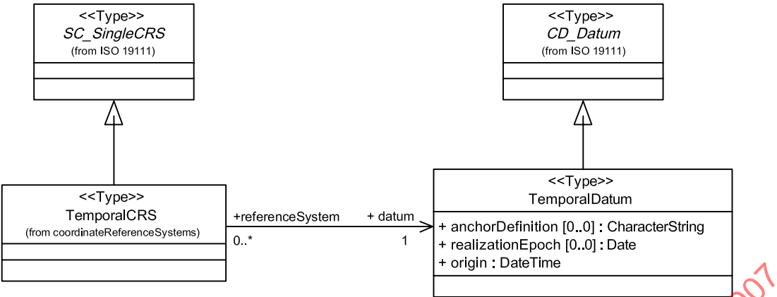
Figure D.54 — Association between TemporalCRS and TemporalDatum
