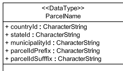
Figure E.4 — A data type &lt;informative&gt;
