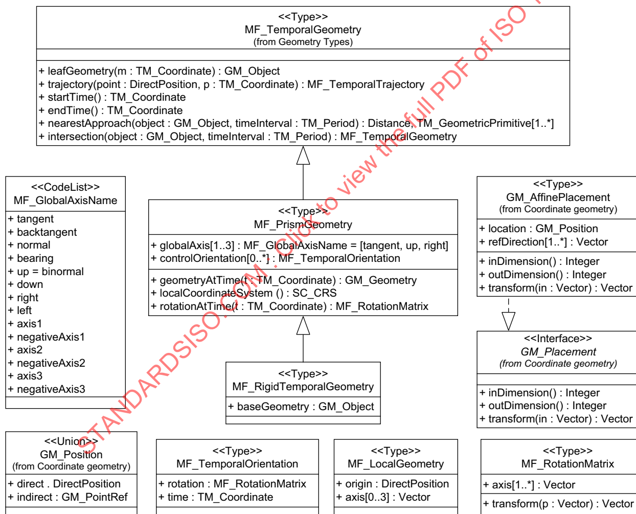
Figure 13 — Classes of the Prism Geometry package
