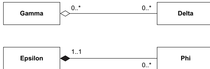
Figure B.5 — Aggregation and Composition
