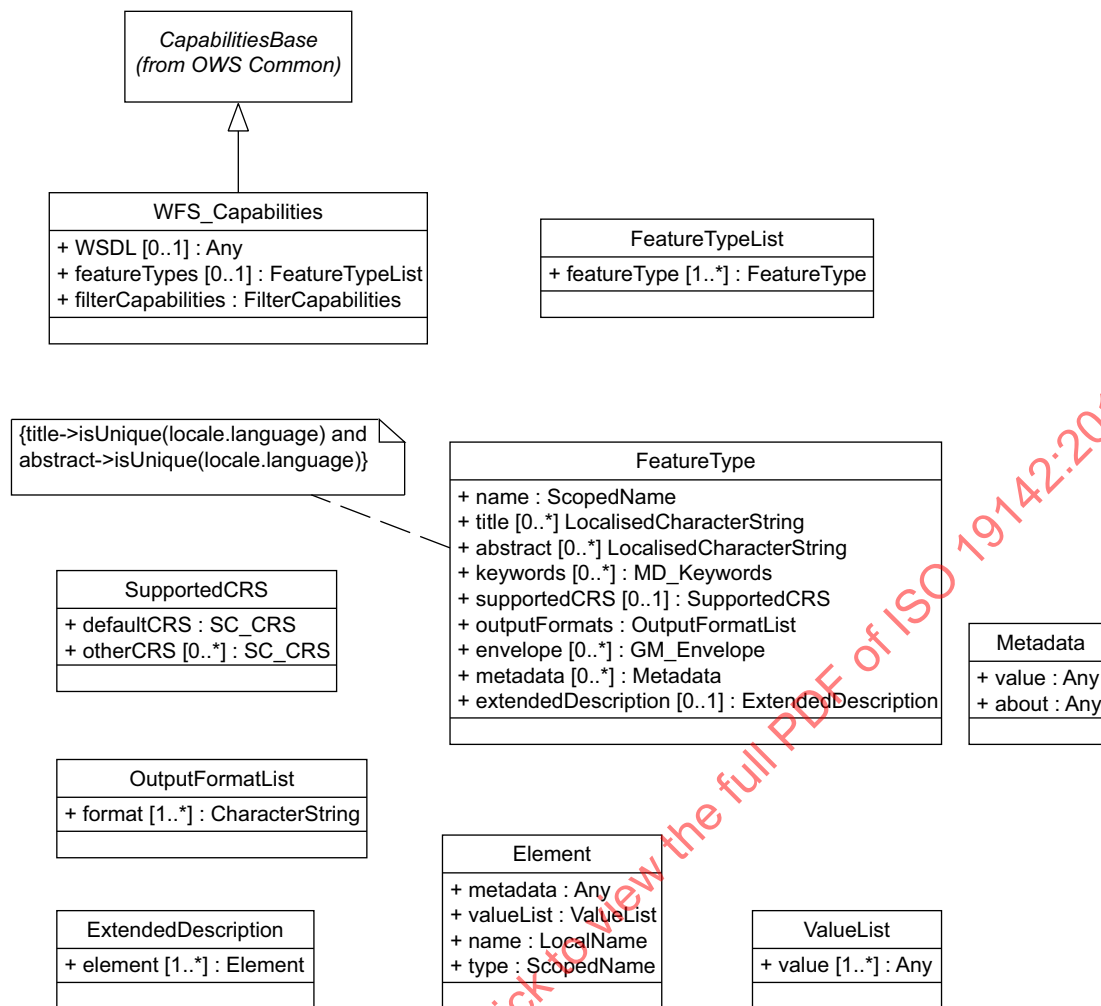
Figure 13 — GetCapabilities response
