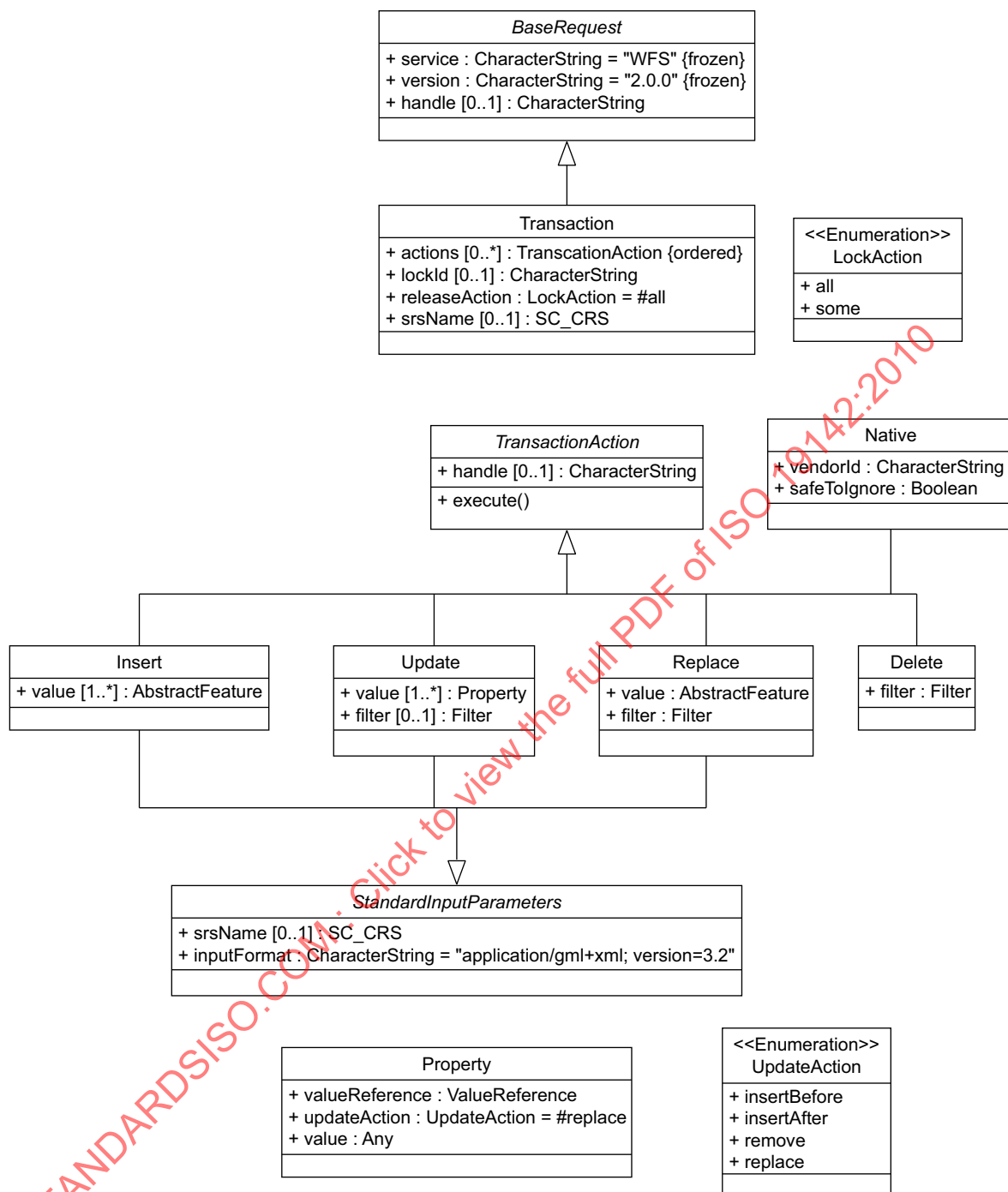
Figure 30 — Transaction request
