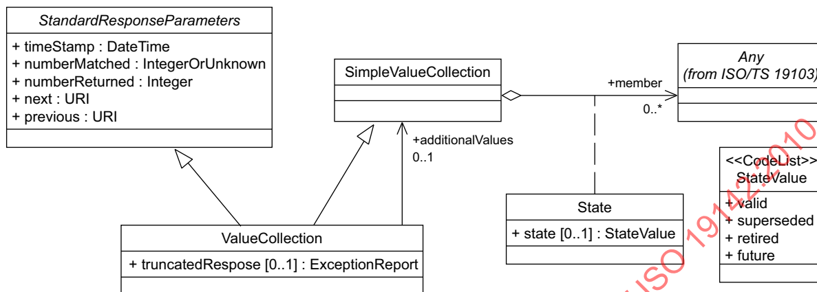
Figure 16 — GetPropertyValue response
