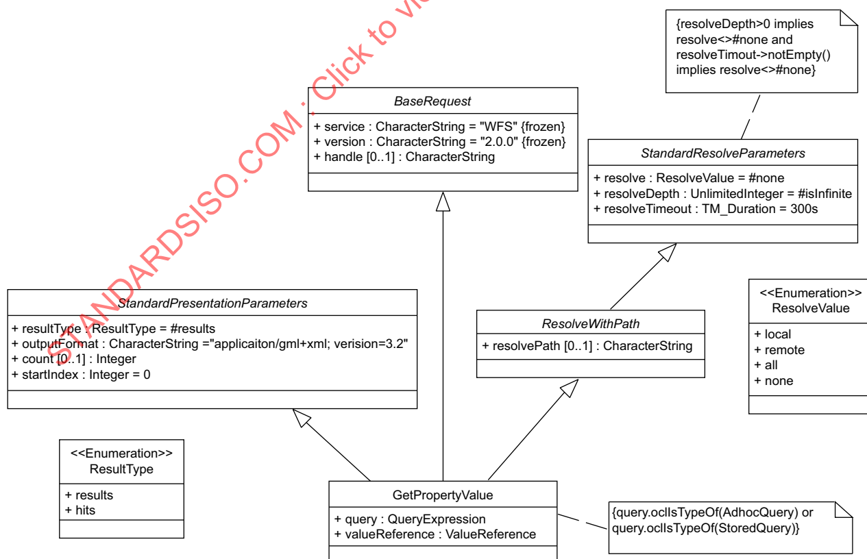
Figure 15 — GetPropertyValue request
