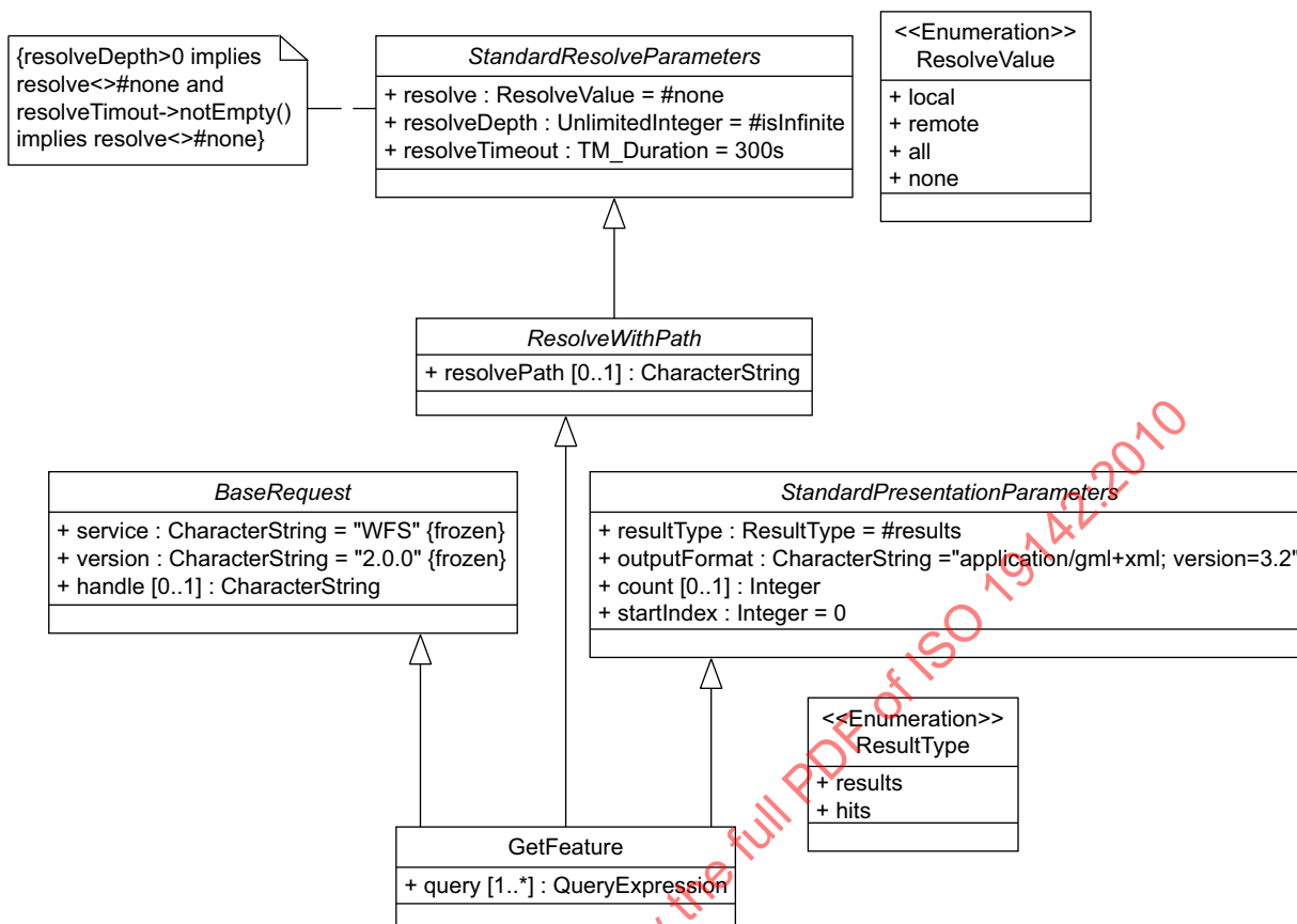
Figure 17 — GetFeature request
