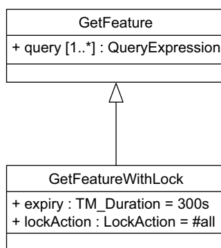
Figure 22 — GetFeatureWithLock request
