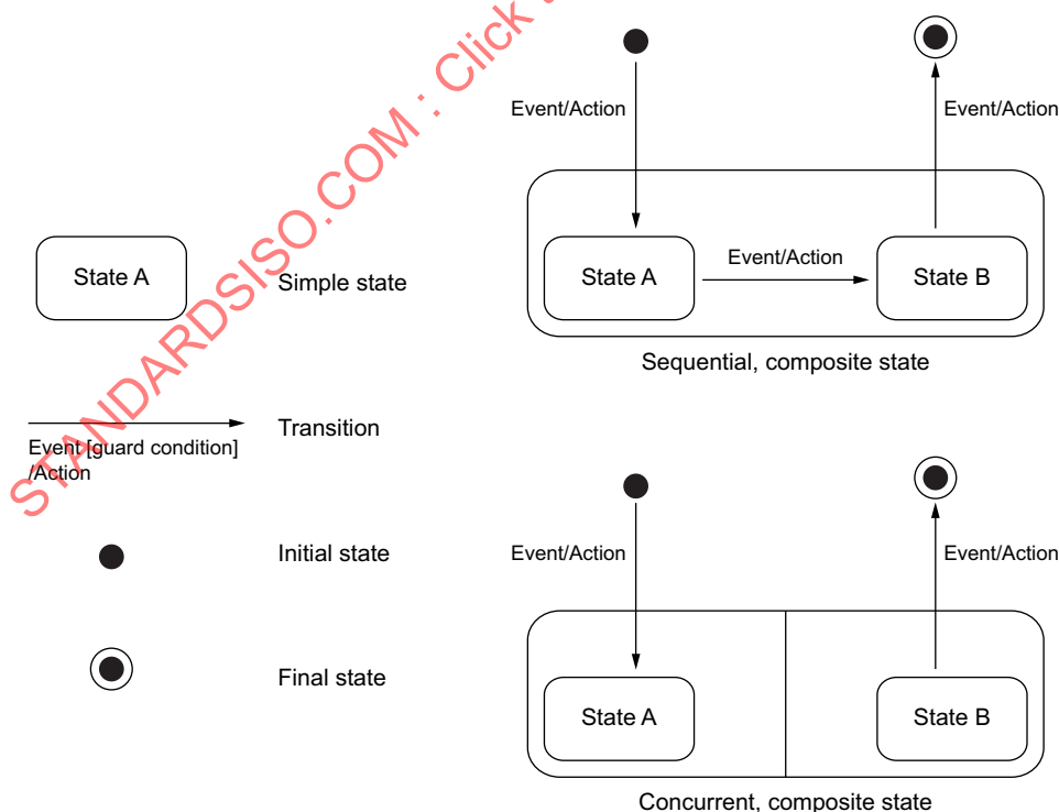
Figure 2 — Summary of UML state diagram notations
