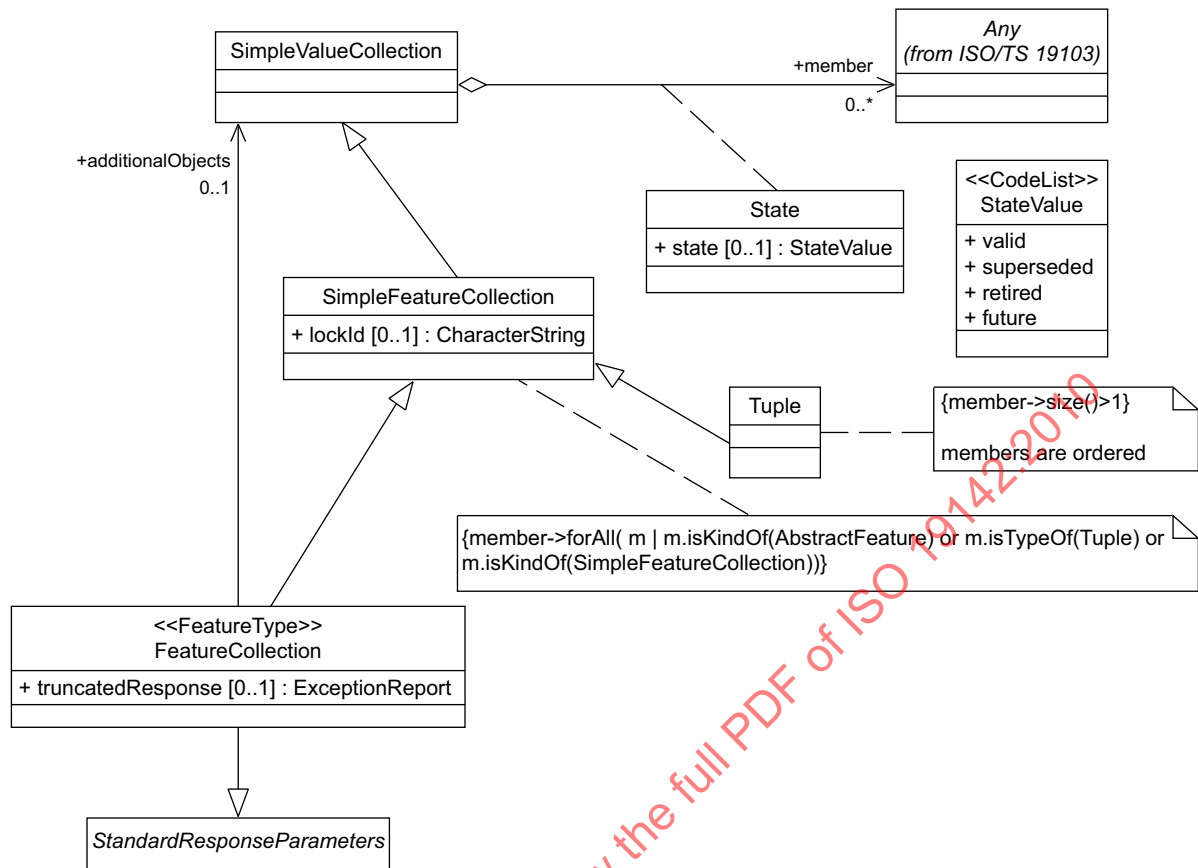
Figure 18 — GetFeature response
