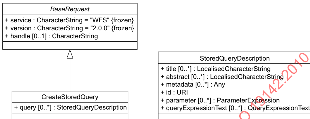
Figure 27 — CreateStoredQuery request
