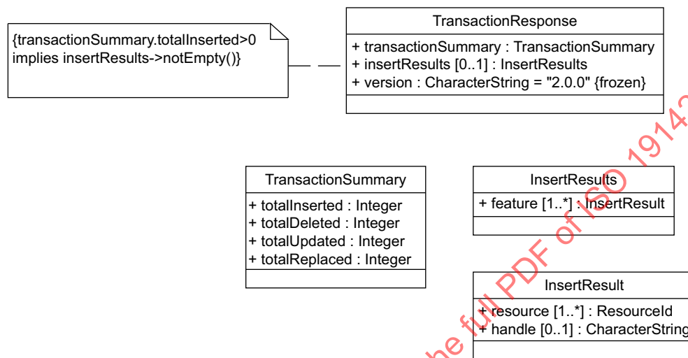
Figure 31 — Transaction response
