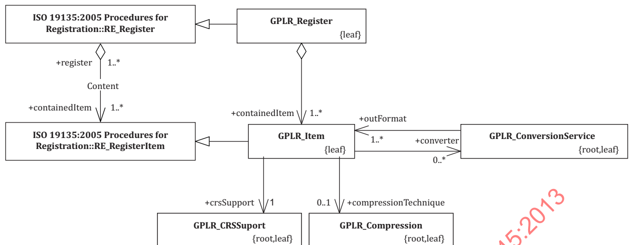
Figure 3 — Overview of the UML GPLR register's schema
