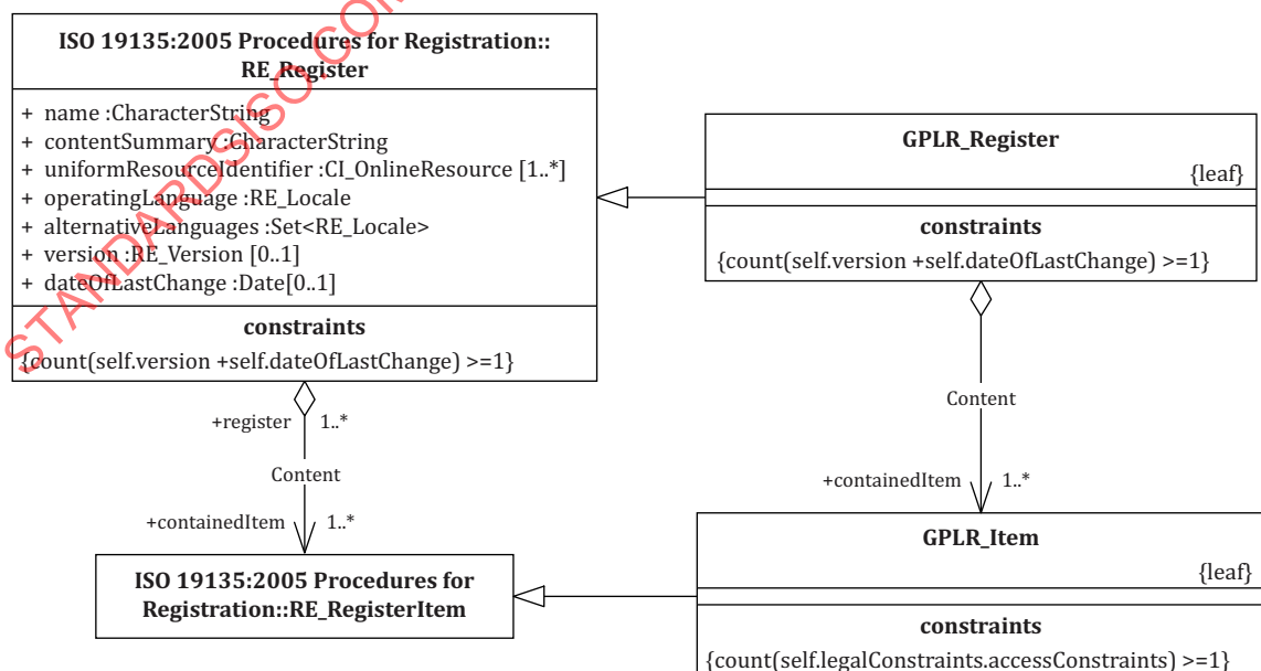
Figure 4 — GPLR_Register
