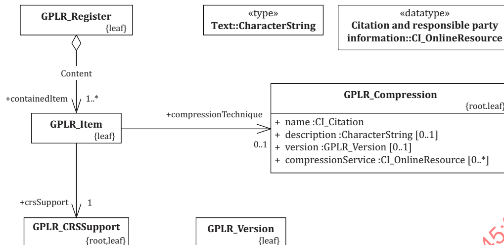
Figure 9 — GPLR_Compression
