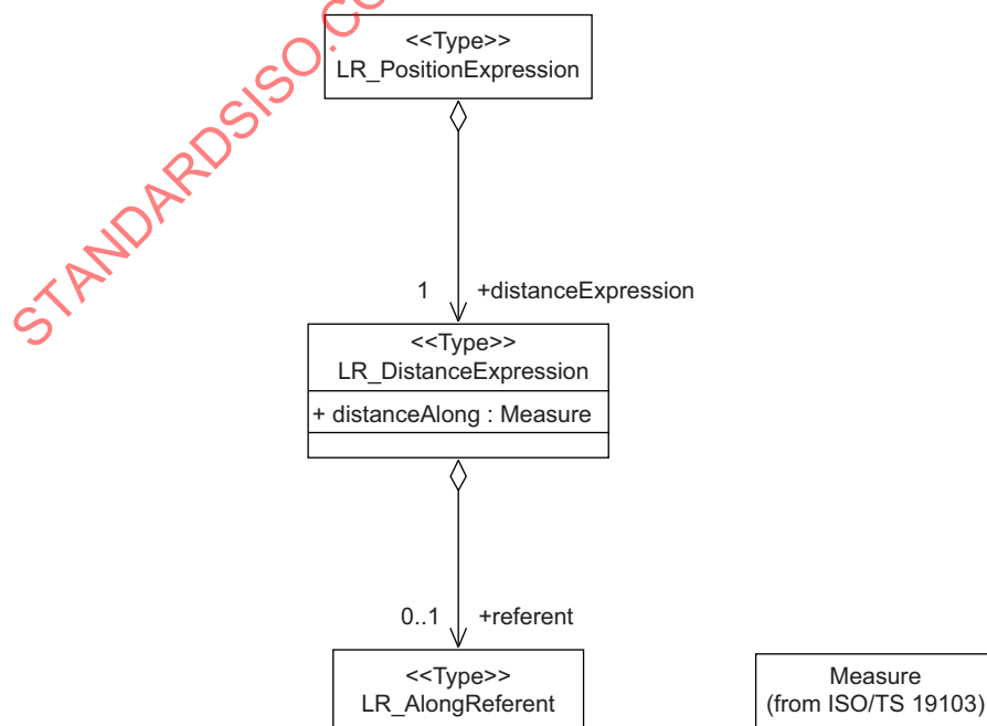
Figure 25 — Context diagram: LR_DistanceExpression
