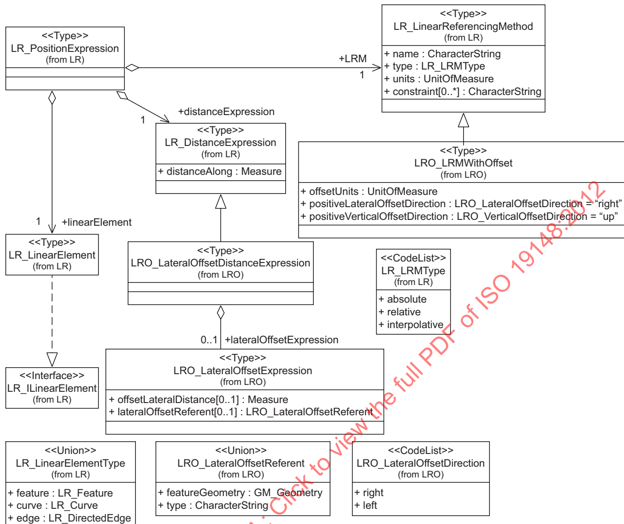
Figure C.3 — Linear referencing system classes for the milepoint with lateral offsets in feet LRM
