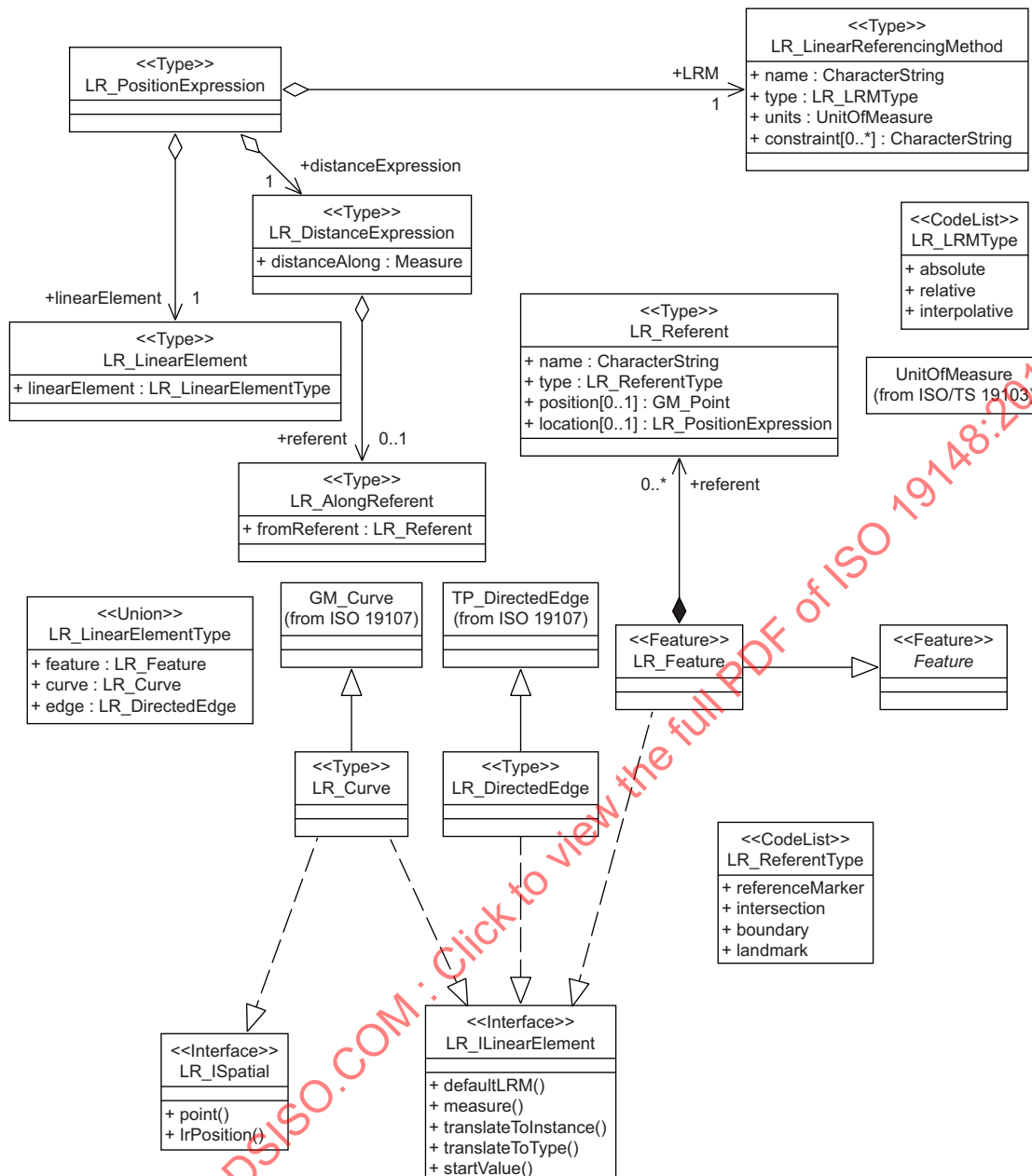
Figure 14 — Linear Referencing System classes
