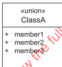
Figure 8 — UML UNION notation
